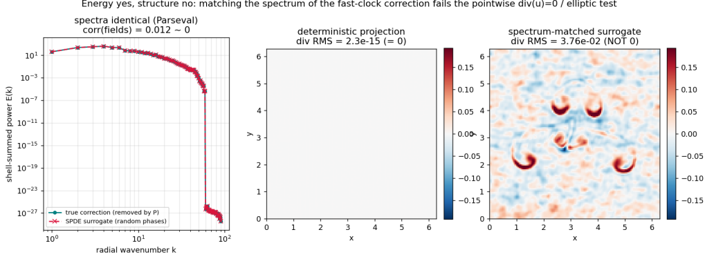
Figure 11: Spectrum-matched surrogate test. A phase-randomized field with the identical power spectrum as the true projection correction (Parseval-exact) fails to reproduce the correction point-wise: ensemble-median correlation |r| = 0.07 ( n = 100 ), and the divergence constraint is left unrepaired ( \text{RMS } \nabla \cdot \mathbf{u} = 3.7 \times 10^{-2} , compared to 2 \times 10^{-15} for the true projection).
