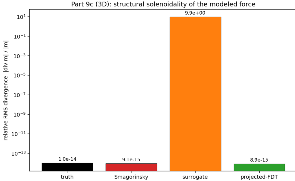
FIG. 6. 3-D solenoidality RMS(\nabla \cdot m) : truth, Smagorinsky and projected-FDT are divergence-free to machine precision (all Leray-projected); the spectrum-matched surrogate fails (phase randomisation breaks \nabla \cdot m = 0 ).
