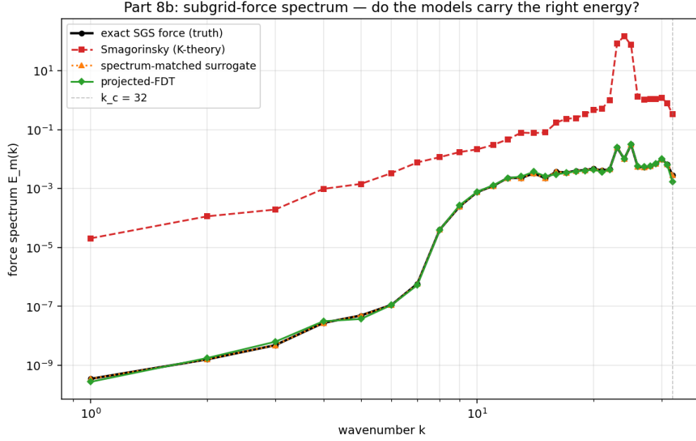
FIG. 1. Subgrid-force spectrum on the 256^2 frozen-field benchmark (sharp-spectral filter at cutoff k_c = 32 ). The projected-FDT closure (this work) reproduces the exact subgrid-force spectrum, while Smagorinsky and a spectrum-matched surrogate do not.
