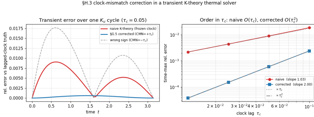
FIG. 10. Transient-solver demonstration of the clock-mismatch correction. The +\tau_c -corrected K-theory solver cuts transient error by about 15\times relative to naive K-theory and vanishes identically in steady turbulence; the -\tau_c sign performs worse than naive, pinning the sign.
