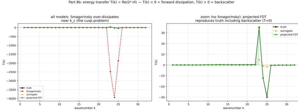
FIG. 3. Energy-transfer spectrum T(k) : negative is forward dissipation, positive is backscatter. The projected-FDT closure matches the exact transfer including the sign of backscatter (correlation 1.000); Smagorinsky is purely dissipative (correlation 0.071).
