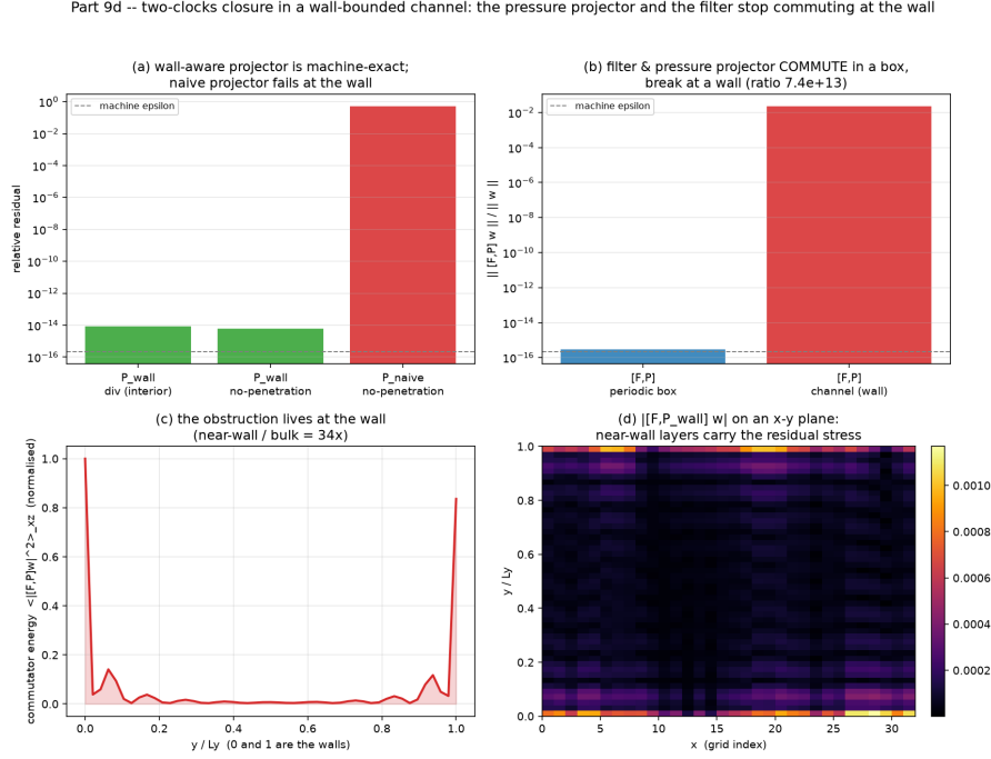
FIG. 9. Wall-bounded a-priori test. The filter–projector commutator [F, \mathbb{P}] is machine-zero in the periodic box but O(10^{-2}) in the channel, peaking at the wall ( 34\times the bulk): a global-pressure (elliptic-clock) correction confined to the near-wall layer, structurally invisible to a local eddy viscosity.
