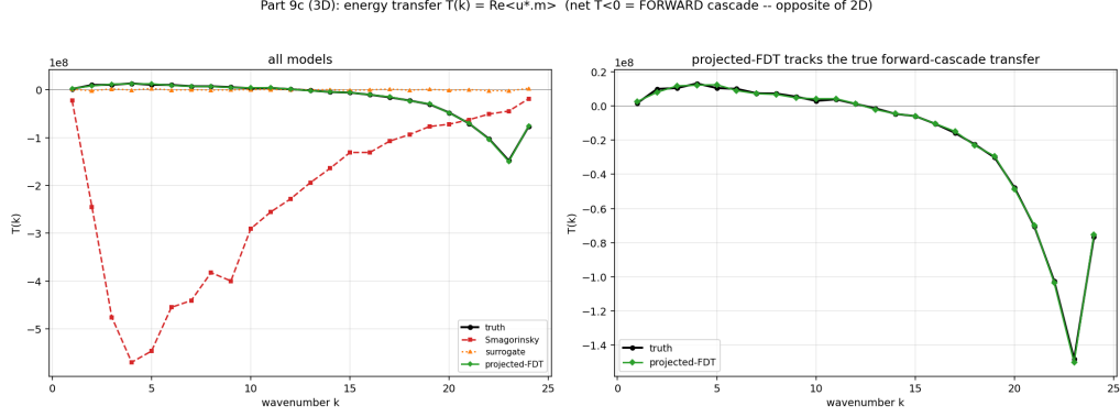
FIG. 7. 3-D energy-transfer spectrum T(k) : net forward cascade; projected-FDT tracks the true transfer (corr 1.000), the surrogate is weakly correlated (0.27), and Smagorinsky is anti-correlated (-0.64).
