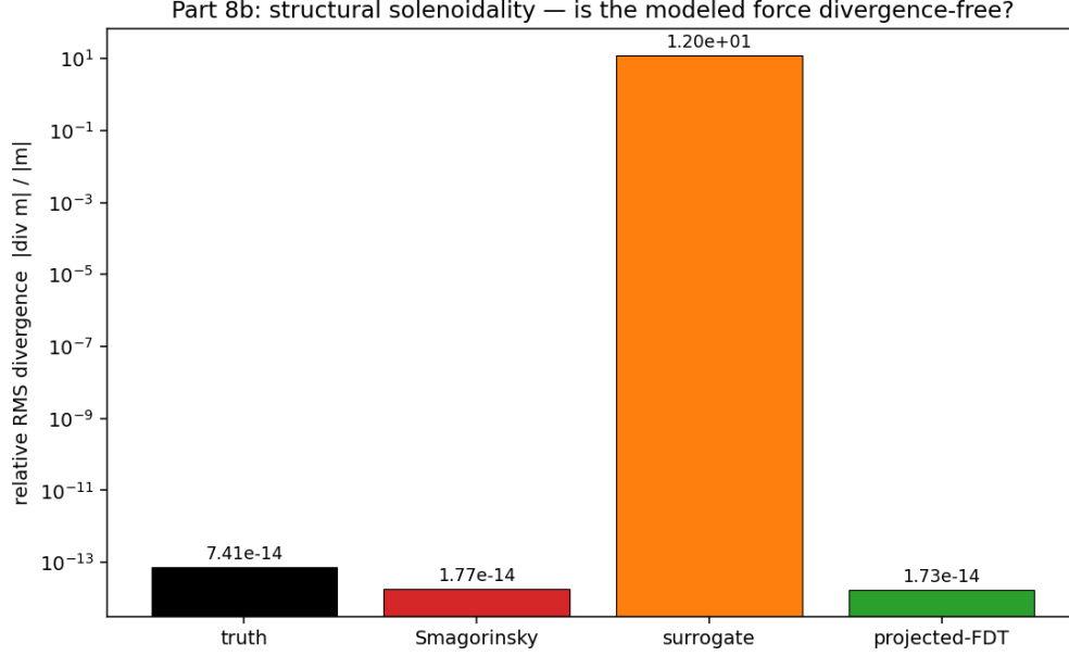
FIG. 2. Solenoidality of the closed subgrid force, the RMS of its divergence. The projected-FDT model stays divergence-free to about 10^{-14} , whereas the spectrum-matched surrogate breaks incompressibility by about 10^1 .
