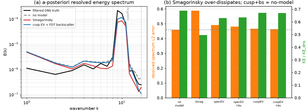
FIG. 4. A-posteriori coarse-LES statistics under each predictive closure versus the spectrally-filtered 256^2 DNS truth (strong-subgrid cutoff). (a) Time-averaged resolved energy spectrum: Smagorinsky (red) over-drains the resolved band, while the cusp eddy viscosity with FDT backscatter (blue) tracks the filtered DNS and nearly matches the no-model spectrum. (b) Resolved-spectrum L2 error and KE/KE_{dns} across closures: every eddy-viscosity closure is stable, Smagorinsky is the most over-dissipative, and the structured cusp+backscatter closure matches (does not beat) no-model — the honest 2-D ceiling.
