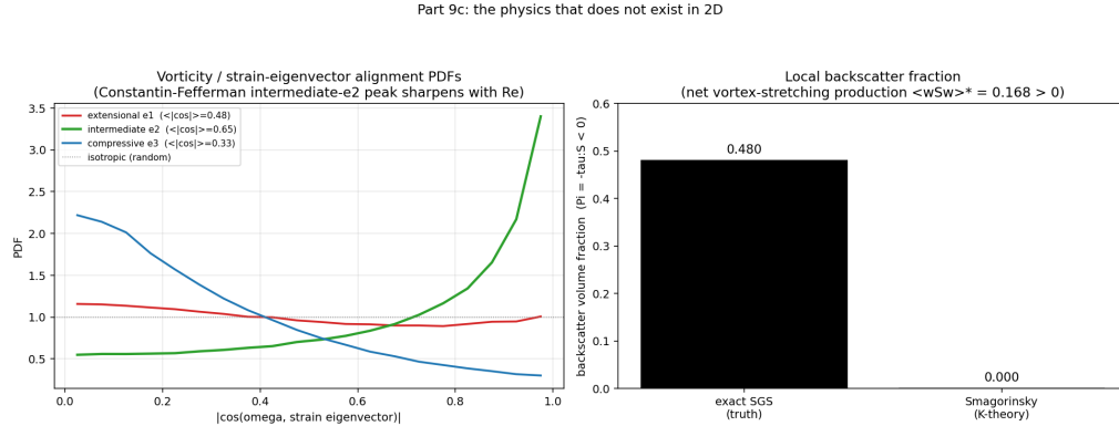
FIG. 8. 3-D-only physics: vortex-stretching production ( > 0 , zero in 2-D), the intermediate-eigenvector strain–vorticity alignment, and the local SGS energy flux \Pi whose backscatter ( \Pi < 0 ) fills \sim 48\% of the volume for the truth and exactly 0\% for Smagorinsky.
