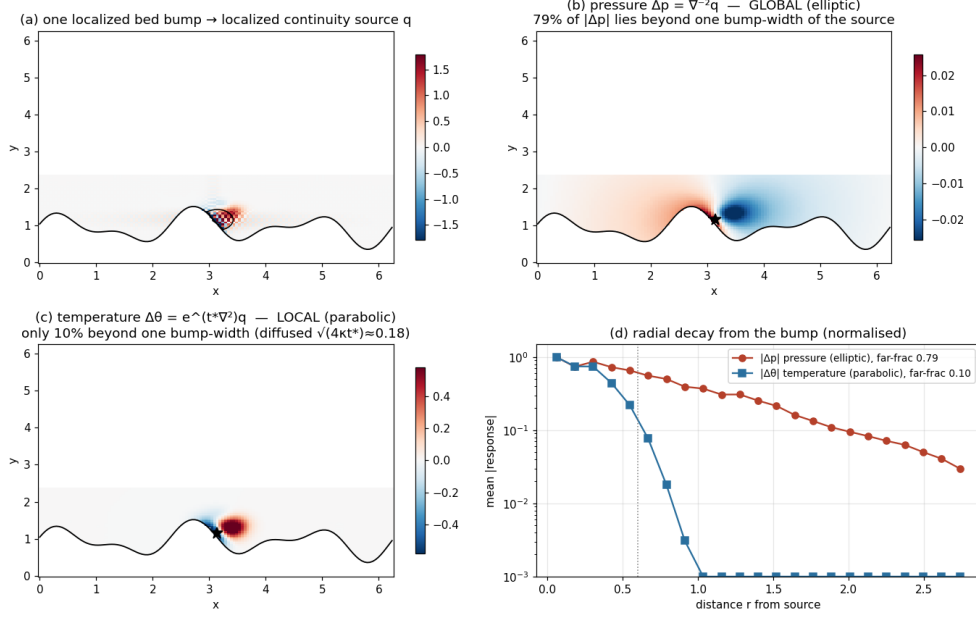
FIG. 5. Response to an identical localized source applied to both operators. The elliptic (pressure) response spreads globally, with 79% of its magnitude beyond one source-width. The parabolic (heat-kernel) response remains confined.
