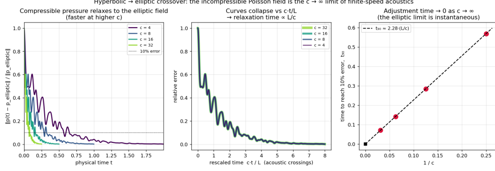
FIG. 6. Relaxation of the compressible pressure field to the elliptic (Poisson) solution for several sound speeds. All curves collapse in the rescaled time ct/L , with t_{90} \approx 2.3 L/c .
