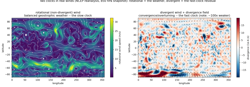
FIG. 11. NCEP/NCAR winds, one analysis day. Left: rotational wind (synoptic highs, lows, and jets). Right: divergent wind (weak, confined to convergence and overturning zones).
