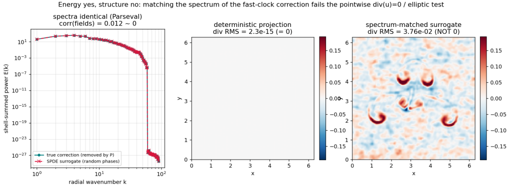
FIG. 10. Spectrum-matched surrogate test. A phase-randomized field with the identical power spectrum as the true projection correction (Parseval-exact) fails to reproduce the correction pointwise: ensemble-median correlation |r| = 0.07 ( n = 100 ), and the divergence constraint is left unrepaired (RMS \nabla \cdot \mathbf{u} = 3.7 \times 10^{-2} , compared to 2 \times 10^{-15} for the true projection).
