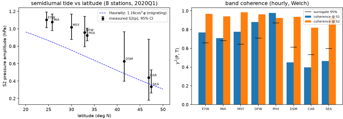
FIG. 2. Left: semidiurnal pressure-tide amplitude versus latitude at eight ASOS stations with bootstrap 95% confidence intervals, compared to the Haurwitz migrating-tide climatology (dashed curve). The monotonic equator-to-pole decay is the signature of a global resonance. Right: band-resolved coherence between hourly pressure and temperature — high at the shared solar lines, at the surrogate noise floor off-line.
