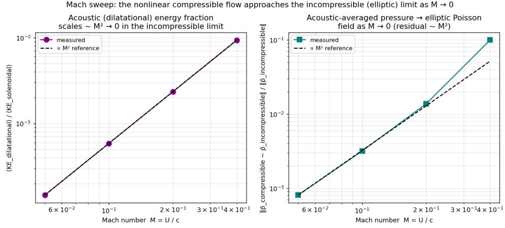
FIG. 8. Mach-number sweep: dilatational energy fraction (circles) and acoustic-averaged pressure residual (squares) both scale as \sim M^2 (dashed line).
