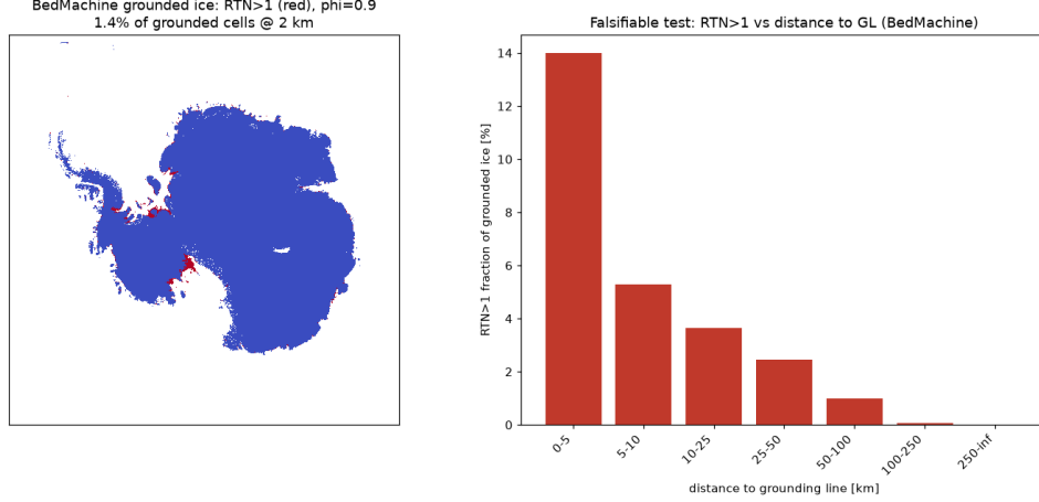
Figure 2: Independent BedMachine Antarctica v4 cross-check at 2 km resolution. The directional result — RTN > 1 concentrated near the grounding line — reproduces the Bedmap2 finding on an independent thickness inversion (median distance-to-grounding-line 6 km for RTN > 1 cells versus \approx 200 km for the rest).
