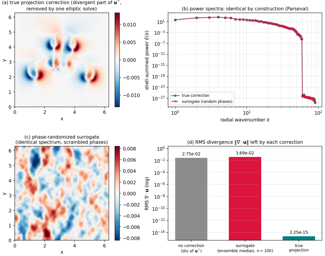
FIG. 1. The surrogate test in one figure. (a) The true projection correction: the divergent part of the intermediate velocity \mathbf{u}^* that a single elliptic solve removes. (b) Power spectra of the true correction and of a phase-randomized surrogate—identical by construction (Parseval-exact). (c) The surrogate correction field: the same spectrum, scrambled phases. (d) RMS divergence left by no correction ( 2.7 \times 10^{-2} ), by the surrogate (ensemble median 3.7 \times 10^{-2} , n = 100 ), and by the true projection ( 2 \times 10^{-15} ). Spectral equivalence is not dynamical equivalence: a field that matches the correction’s power spectrum does not reproduce its action as a constraint.
