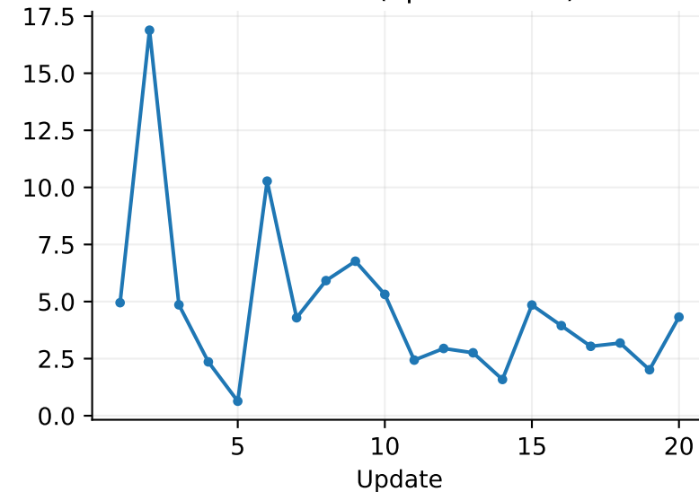
Gradient norms before clipping
