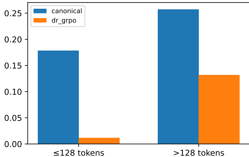
Mean total derivative L1 mass
