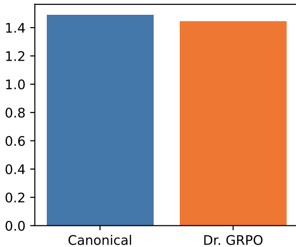
Held-out reward
