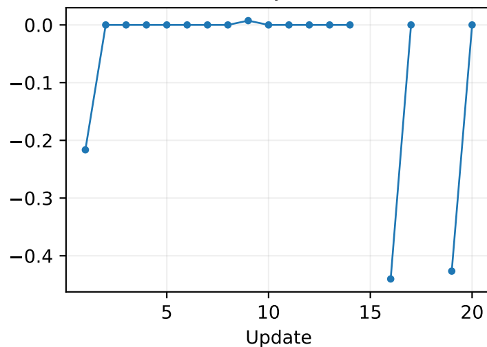
Generation-cap fraction
