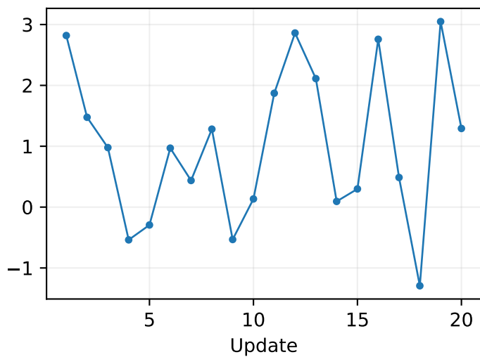
Uninformative-group fraction
