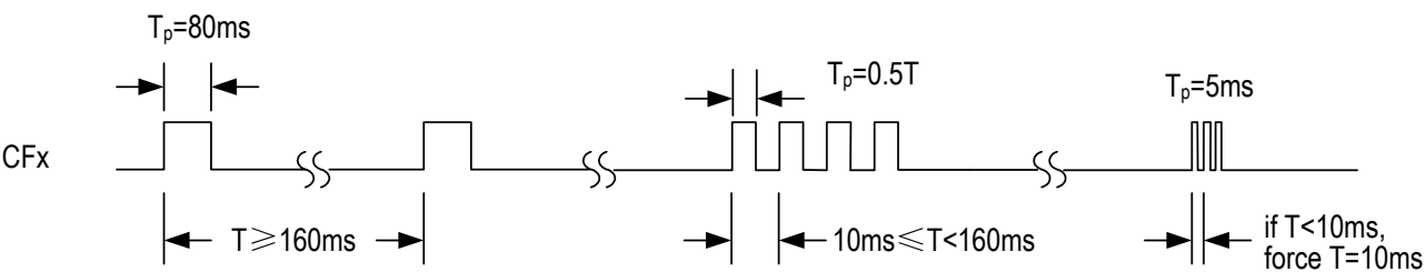
Figure-15 Output Pulse Width
