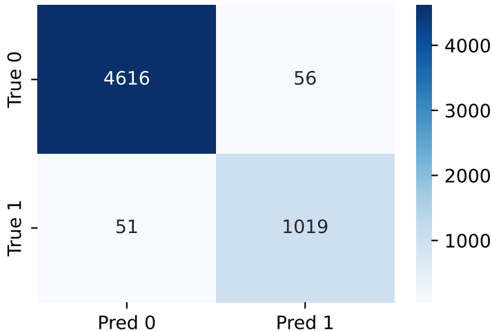
Confusion Matrix — web_aug / dblp-scholar
