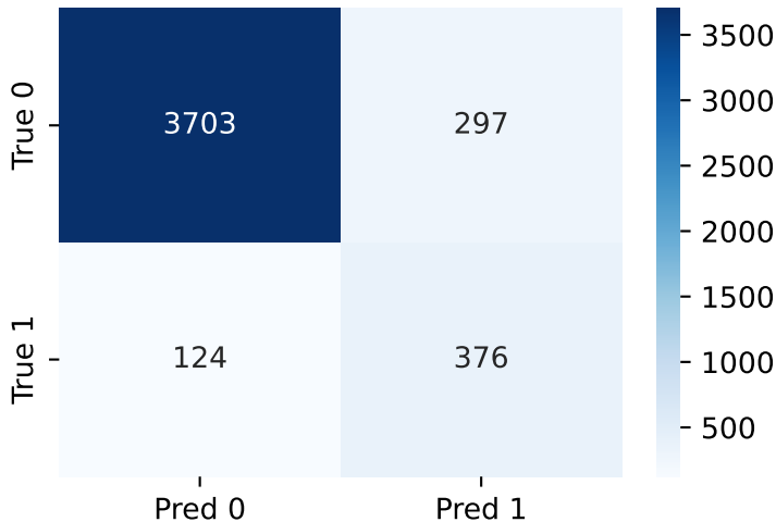
Confusion Matrix — baseline_cw / wdc-products
