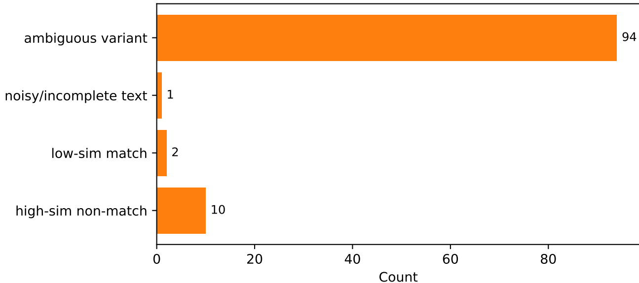
Error classes — web_aug / dblp-scholar
