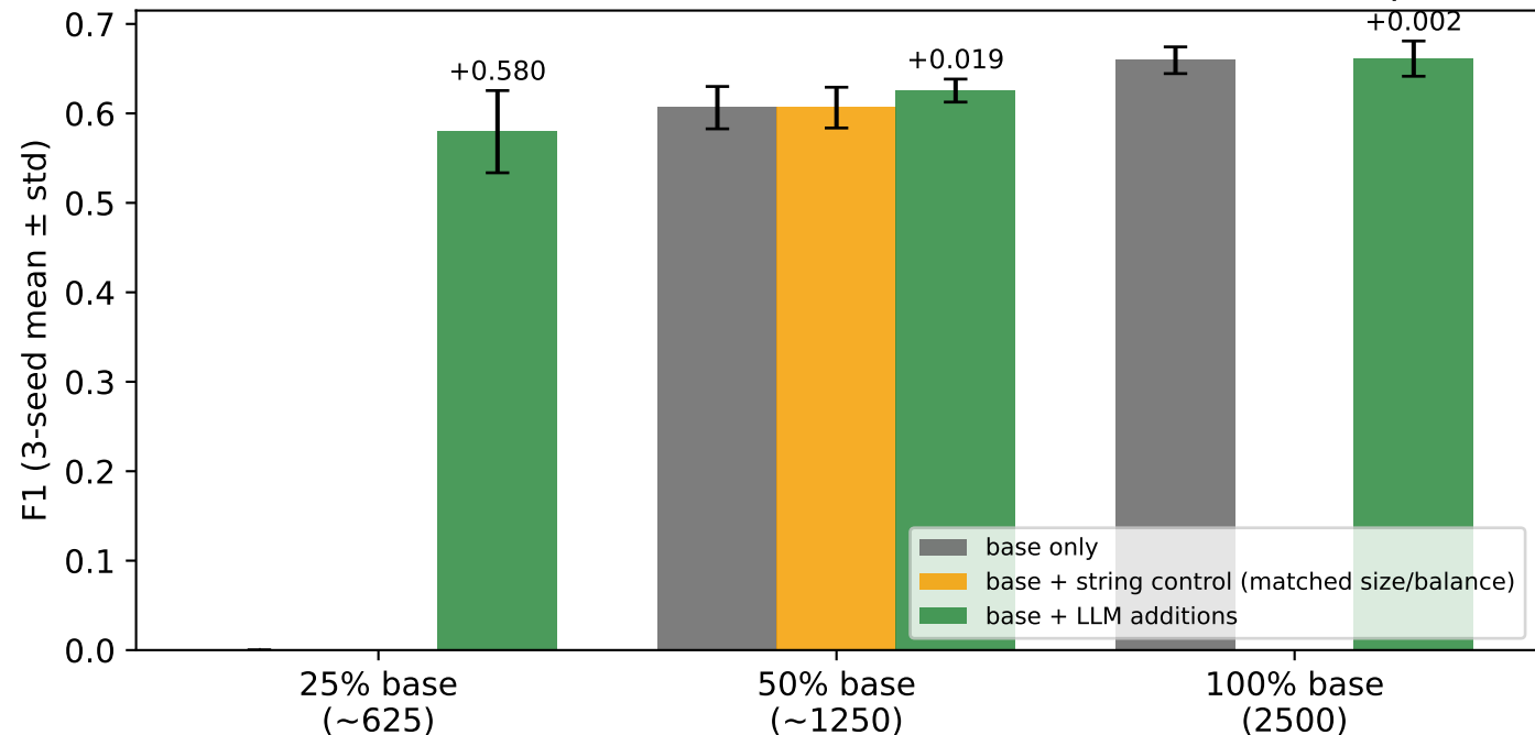
WDC Products: LLM additions vs. base and volume-matched control per budget
