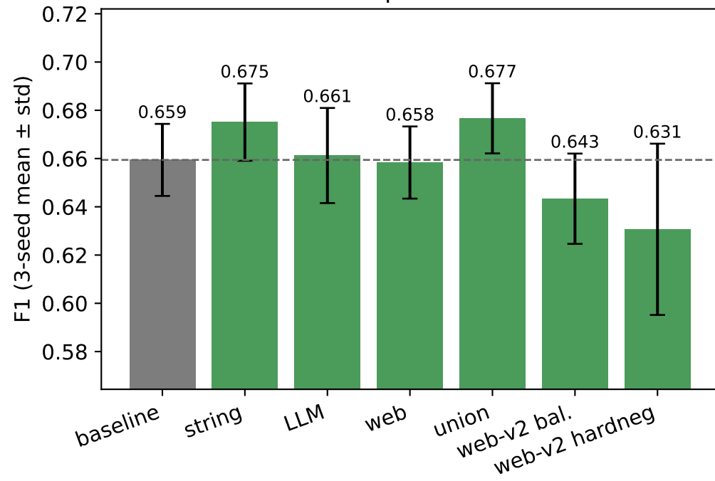
wdc-products
