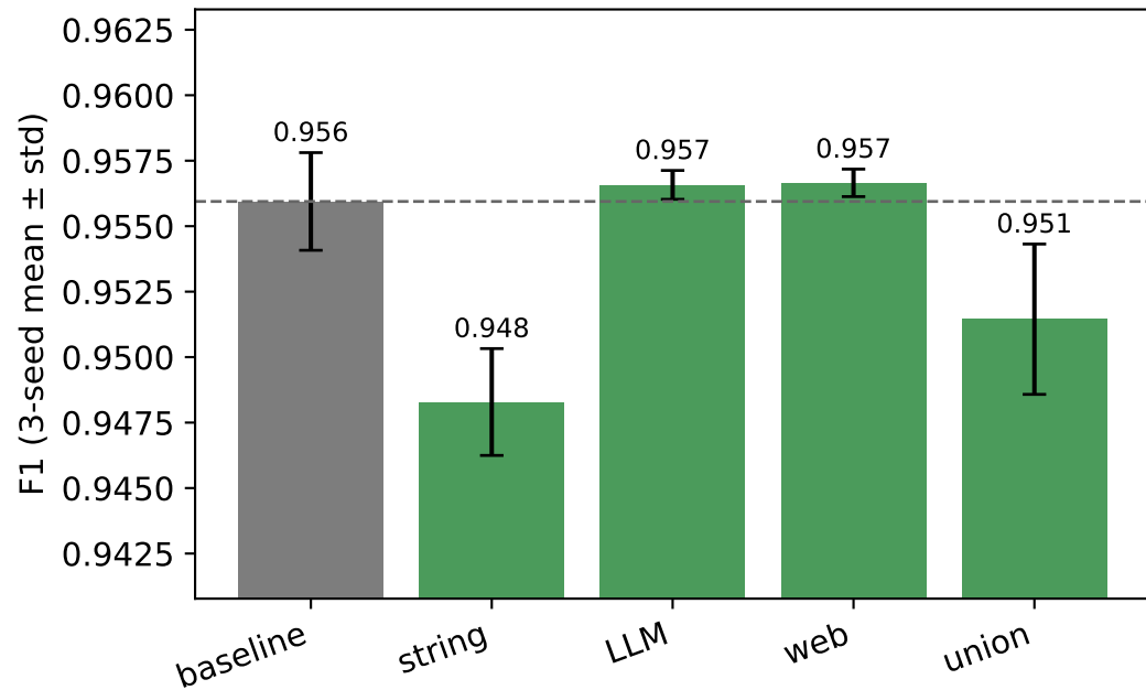
dblp-scholar
