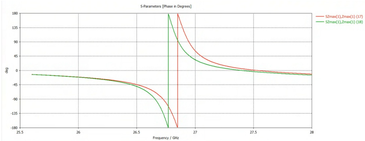
Figure 9. Reflection phase of the co-polarised term SZmax(1),Zmax(1) at the two capacitance endpoints on the current diagnostic geometry (patchW = 2.30 mm, slotL = 2.32 mm, slotW = 0.35 mm, lineV = 1.13 mm), over approximately 25.5 to 28 GHz. Red is varC = 0.19 pF and green is varC = 0.025 pF. Near the intended 26.104 GHz operating frequency the two traces are drawn on top of one another at approximately -24 degrees and no separation is measurable. They become distinguishable at about 26.3 GHz and reach roughly 7 degrees apart at 26.5 GHz and 13 degrees at 26.6 GHz, before each wraps through the rapid transition that accompanies its own resonance: near 26.85 GHz at 0.19 pF and near 26.77 GHz at 0.025 pF. The displayed phase wraps at plus or minus 180 degrees, so the apparent excursion between the two wrap points is an artefact of the display and no tuning range in degrees is quantified from this plot.
