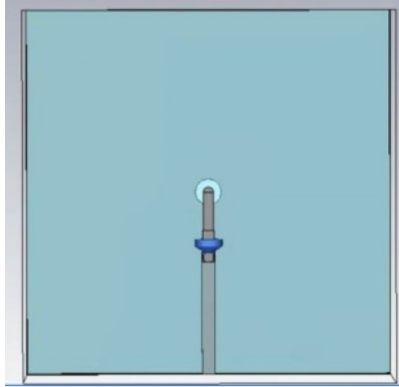
Figure 5. The blind via crossing the layer-four ground plane. The circular clearance around the via, drawn here as the light ring, is what keeps the resonant path isolated from the ground plane as it passes through it. The lumped element representing the varactor is the darker collar on the lower part of the via, at the layer-six terminal pads. The clearance diameter is not published and is a reconstruction assumption; see Appendix F.
