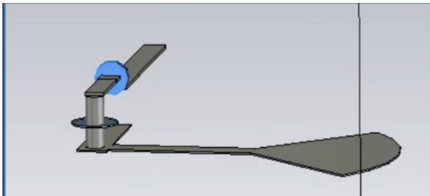
Figure E.4. The bias network of Figure 6 from a second angle, with the ground-plane clearance ring around the blind via more clearly separated from the radial stub.
