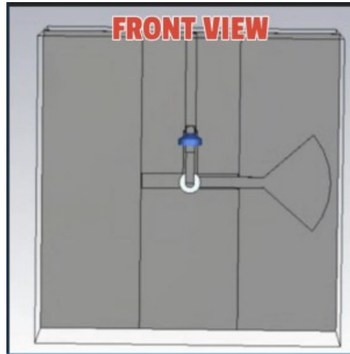
Figure E.2. Front view, looking into the stack along the propagation axis. The layer-three stripline, the blind via, the lumped varactor and the laterally branching radial stub are visible through the semi-transparent conductors. The view label is part of the original screen capture.
