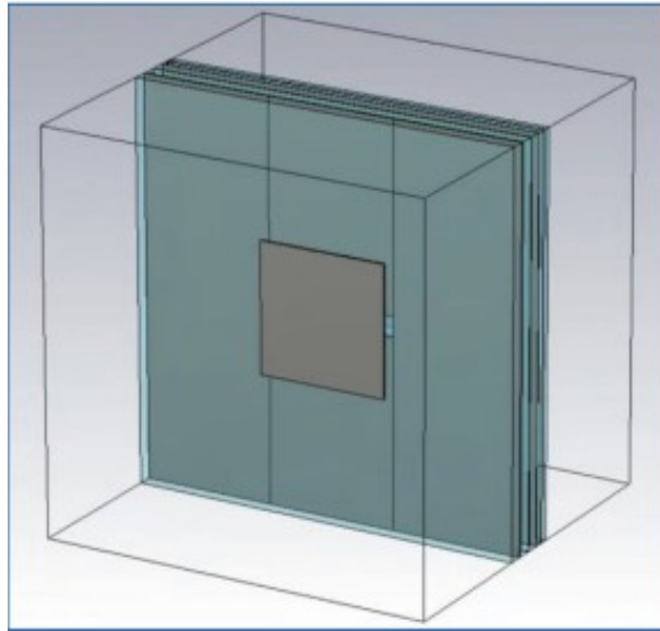
Figure 3. Reconstructed unit cell in CST Studio Suite 2023, shown inside the bounding box of the periodic simulation domain. The model is a 7 mm by 7 mm cell containing six perfect-electric-conductor layers separated by five Astra MT77 substrates, with an ideal lumped capacitor across the layer-six terminal pads representing the varactor. The substrates are drawn semi-transparent and the square layer-one patch is visible on the front face; the open space above and below the stack is the region through which the Floquet excitation enters and leaves.
