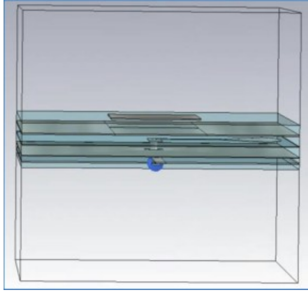
Figure 4. The same model viewed close to edge-on, so that the conductor layers are separated in depth rather than superimposed. Reading downward: the square patch on L1, the L2 conductor interrupted by the rectangular coupling aperture, the L3 stripline with its bias-T branch and radial stub, the L4 ground plane with the circular clearance around the blind via, and the L5 and L6 routing carrying the lumped varactor, visible below the stack. This is a single oblique capture rather than a per-layer exploded set, so the layers are identified by their depth order, not shown in isolation.
