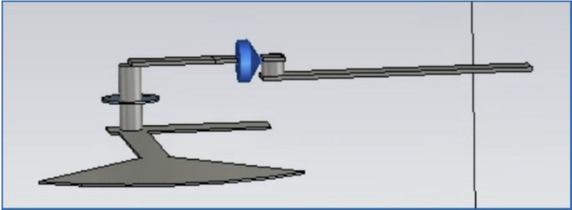
Figure 6. The bias network with the substrates and the sheet conductors hidden, so that the routing can be followed. The blind via descends from the layer-three stripline, through its ground-plane clearance, to the terminal pads carrying the lumped varactor; the bias line continues away from the junction and the radial stub branches laterally from it. This lateral branching, rather than a stub continuing along the bias line, is the reading taken from Figure 1 and supported by Figure D.1.
