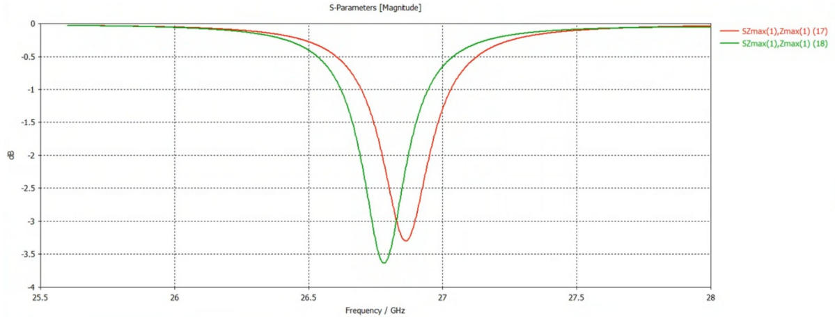
Figure 8. Reflection magnitude of SZmax(1),Zmax(1) at the two capacitance endpoints on the current diagnostic geometry, over approximately 25.5 to 28 GHz. Red is varC = 0.19 pF (run 17) and green is varC = 0.025 pF (run 18). A single resonant dip appears near 26.8 GHz and moves with capacitance: approximately 26.86 GHz and -3.3 dB at 0.19 pF against approximately 26.78 GHz and -3.6 dB at 0.025 pF, a shift of roughly 0.08 GHz. This is the clearest evidence in this project that the varactor reaches the resonance of the complete unit cell. Both figures are read from the plot rather than exported from the solver, and the sweep extends beyond the declared Astra MT77 material fit range of 25.6 to 26.6 GHz, so the region is a diagnostic indication rather than a quantitative prediction.
