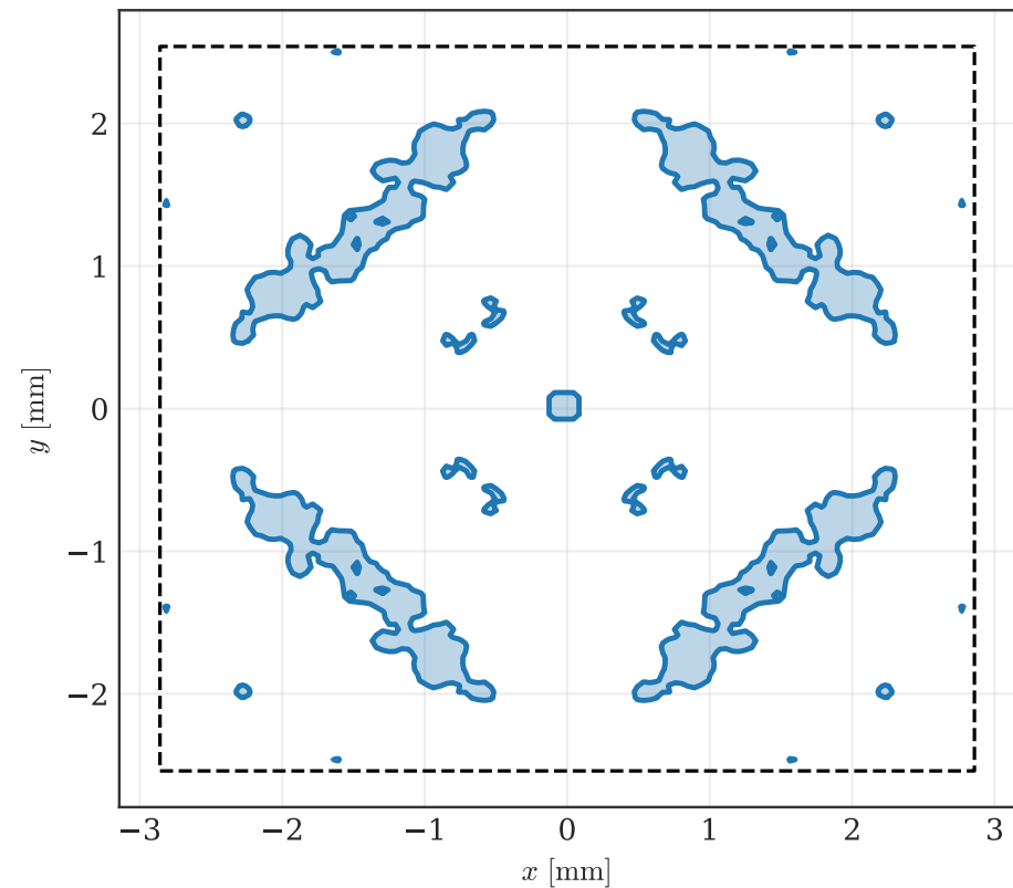
Parametric CAD Vector Layout (Golden Geometry #1)
