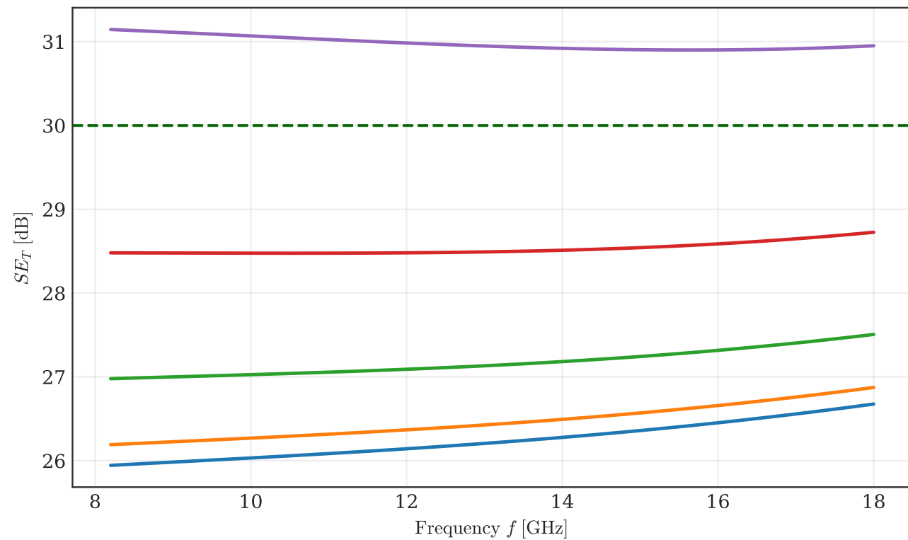
Oblique Incidence Total Shielding SE_T(\theta) vs Frequency
