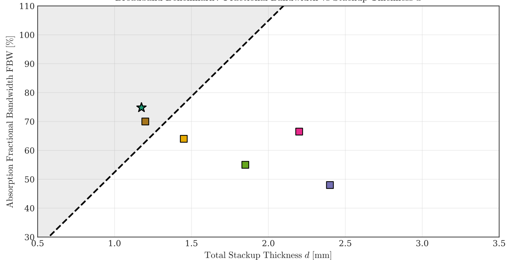
Broadband Benchmark : Fractional Bandwidth vs Stackup Thickness d
