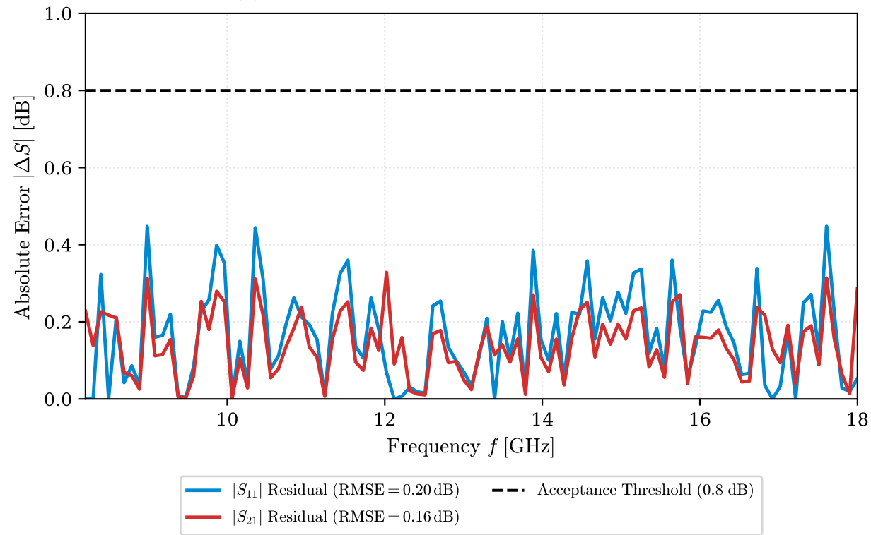
(a) Point-by-Point S-Parameter Residual Errors
