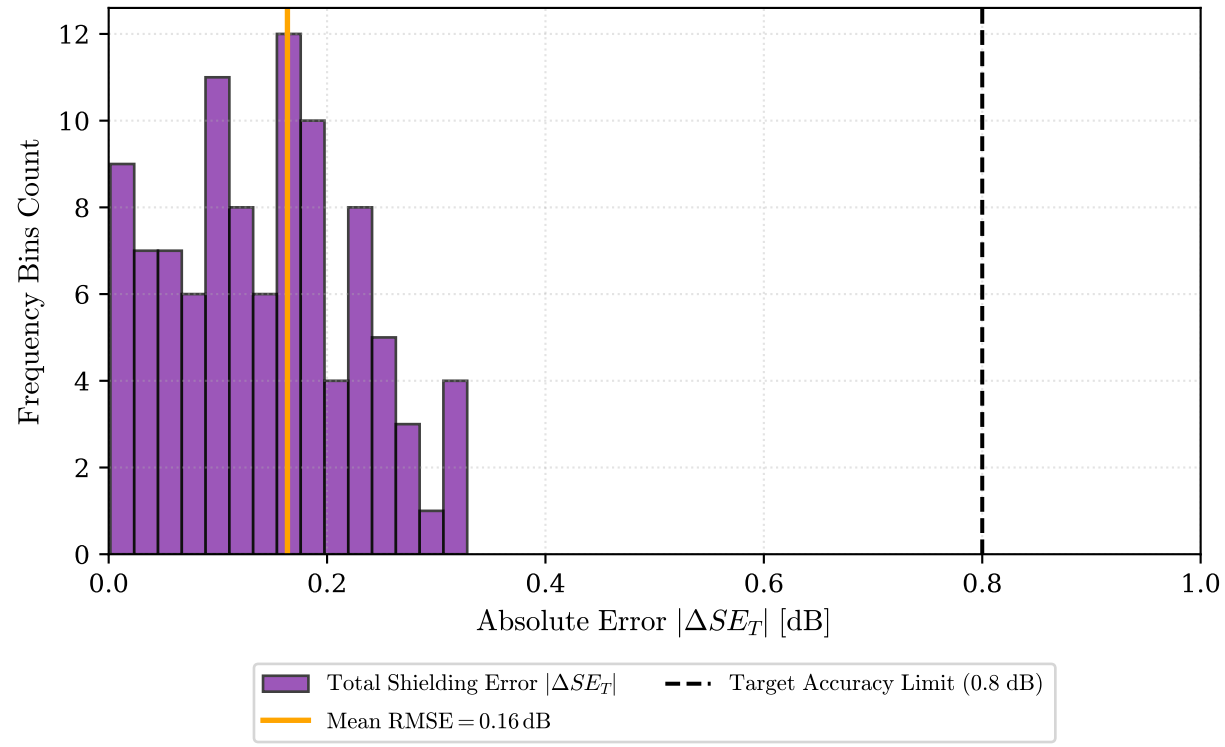
(b) Shielding Effectiveness Error Distribution
