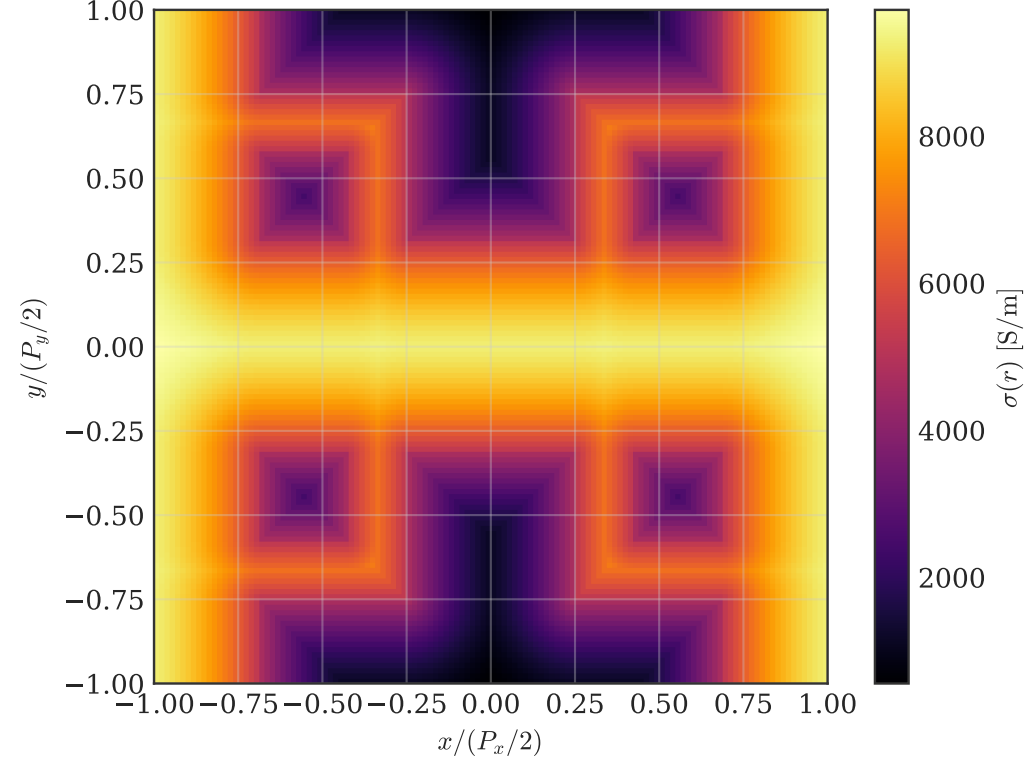
Surface Conductivity \sigma(x, y) [S/m] ( \beta = 4.0 , \sigma_{\text{film}} = 10^4 S/m)
