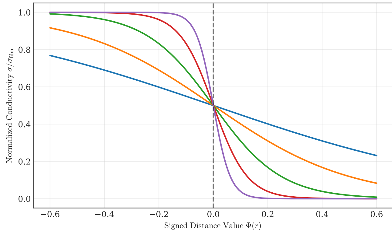
Regularized Heaviside Projection \sigma/\sigma_{\text{film}} vs \Phi(r)
