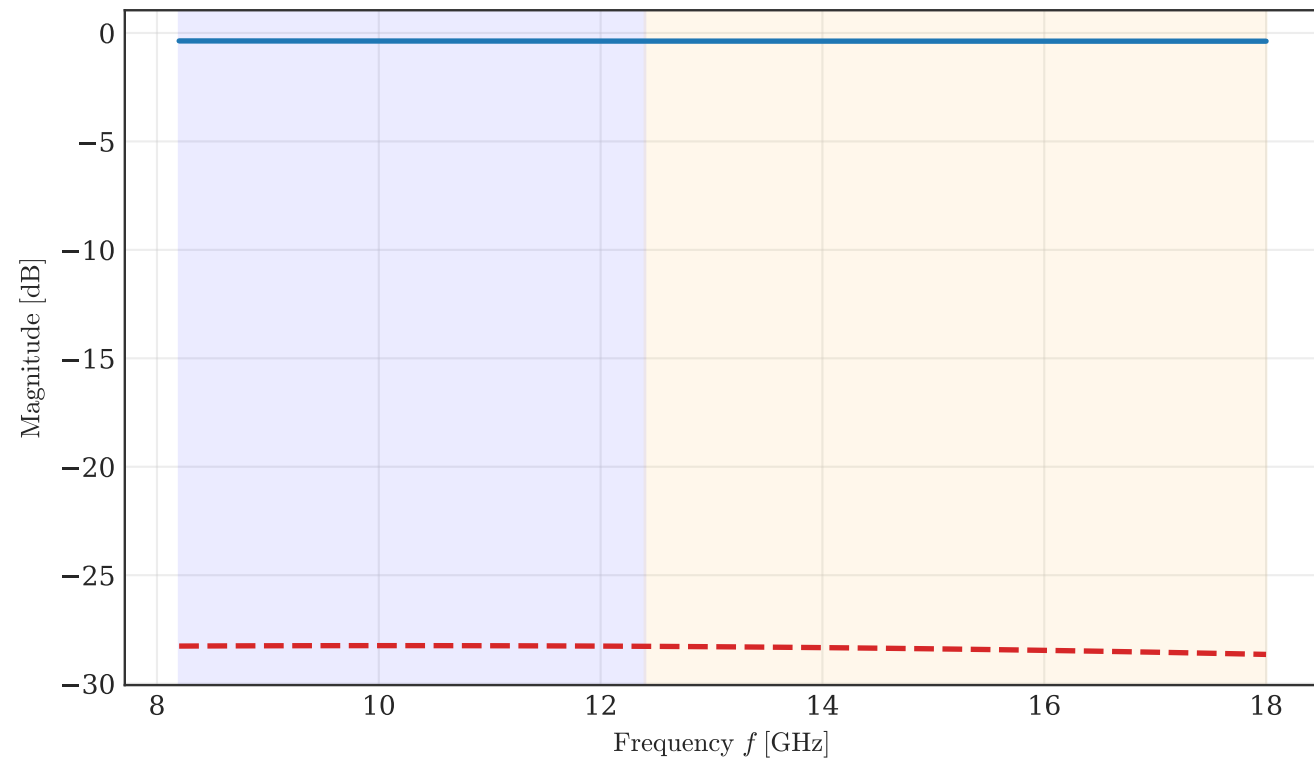
Complex Scattering Parameters ( S_{11} , S_{21} )
