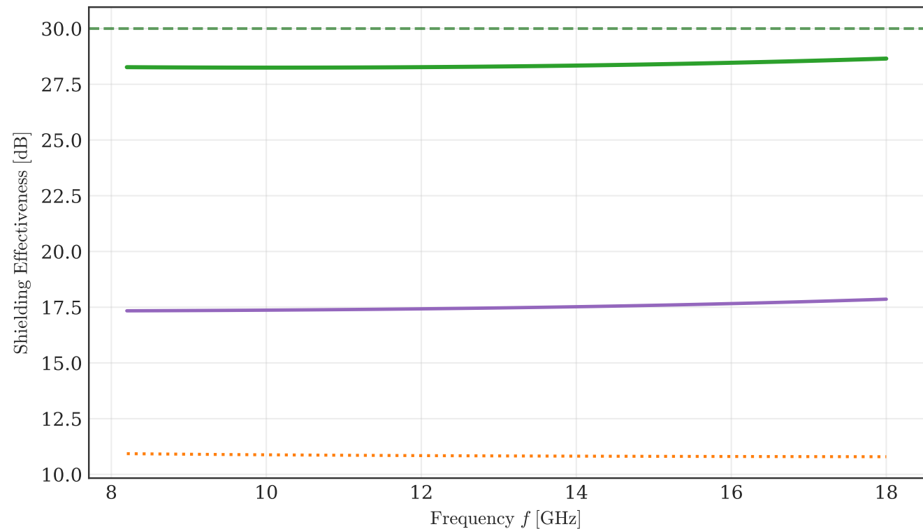
EMI Shielding Effectiveness ( SE_T = SE_A + SE_R )
