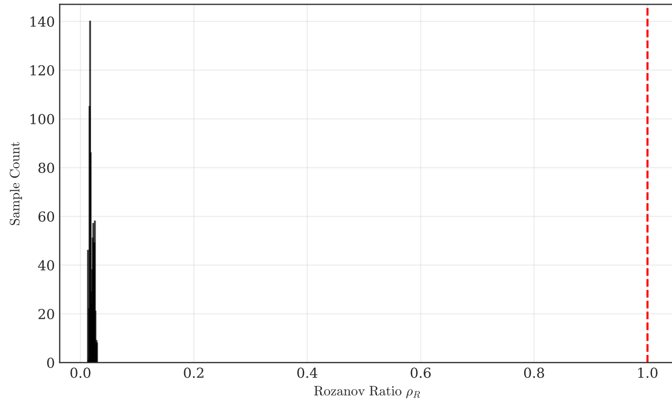
Distribution of Rozanov Figure of Merit ( \rho_R )
