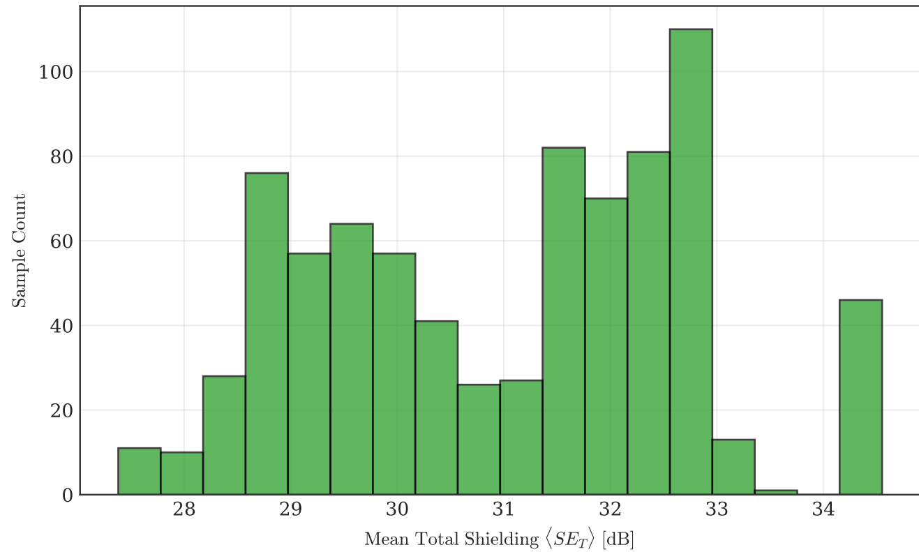
Distribution of Mean Shielding Effectiveness ( \langle SE_T \rangle )
