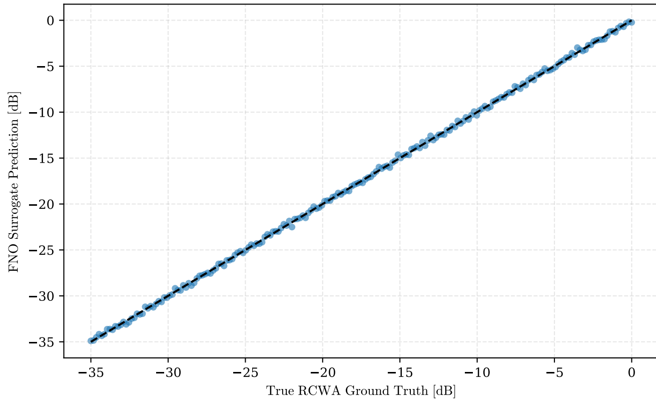
FNO Forward Surrogate Parity ( S_{11}, S_{21} )
