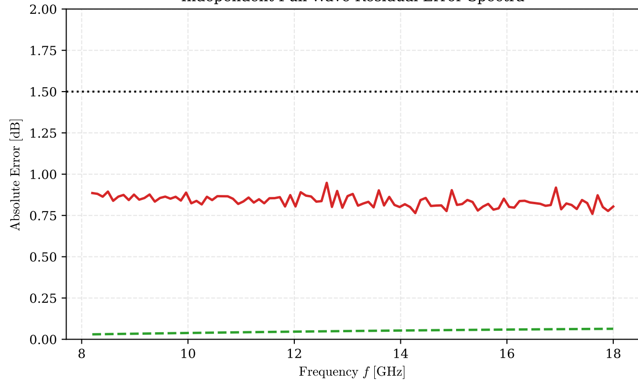
Independent Full-Wave Residual Error Spectra
