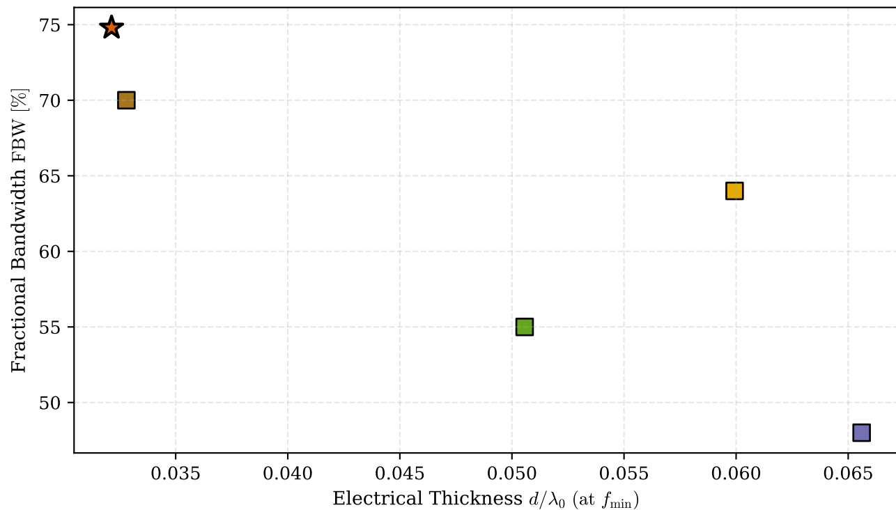
Pareto Frontier: Electrical Thickness vs Bandwidth
