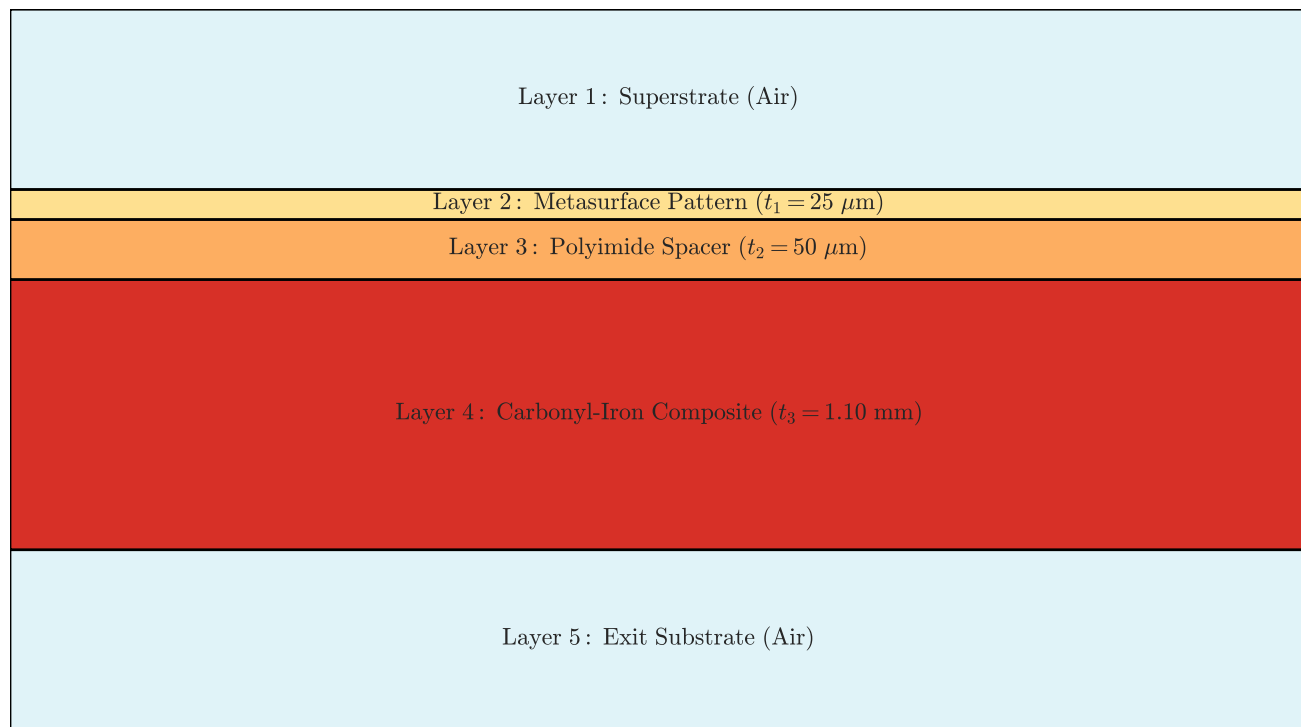
Five-Layer Stratified Composite Stackup ( d = 1.175 mm \leq 1.20 mm)
