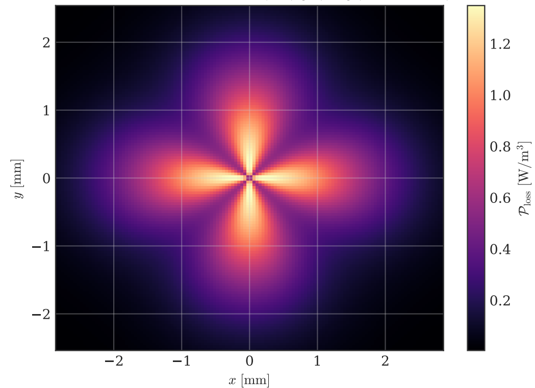
Volume Power Loss Density \mathcal{P}_{\text{loss}}(x, y) [W/m 3 ] ( f = 12.0 GHz)
