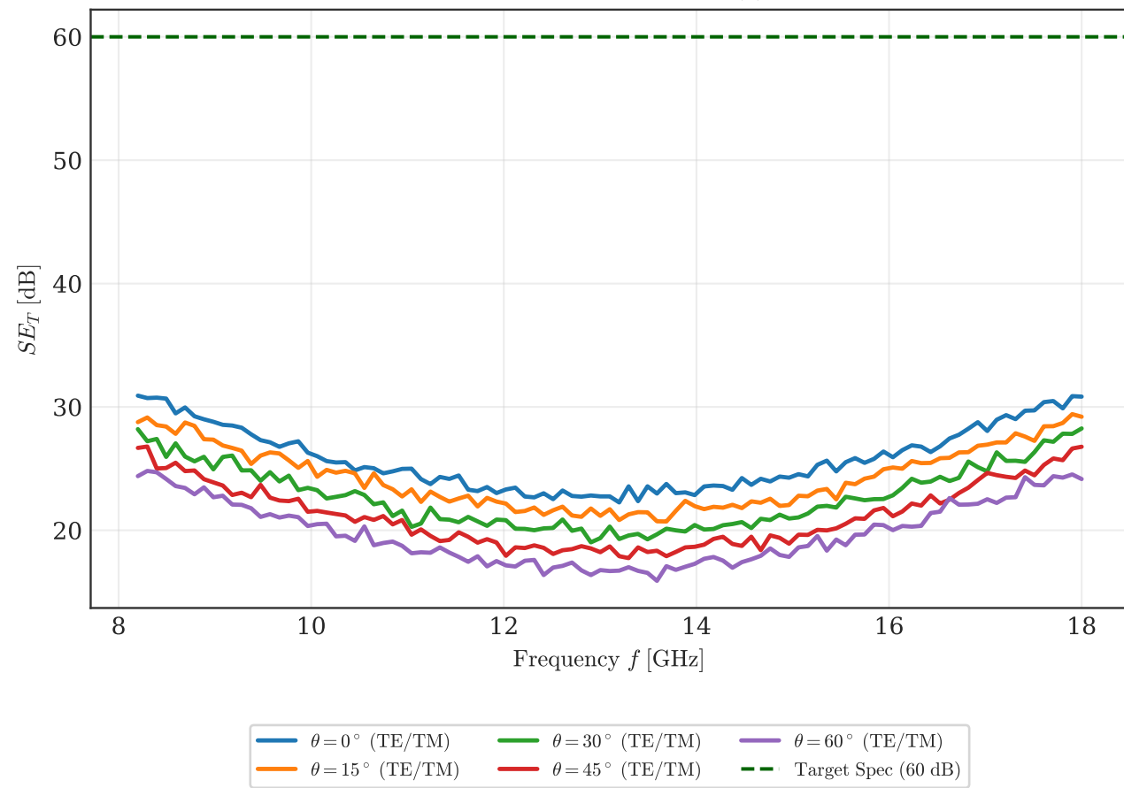
Oblique Incidence Total Shielding SE_T(\theta) vs Frequency
