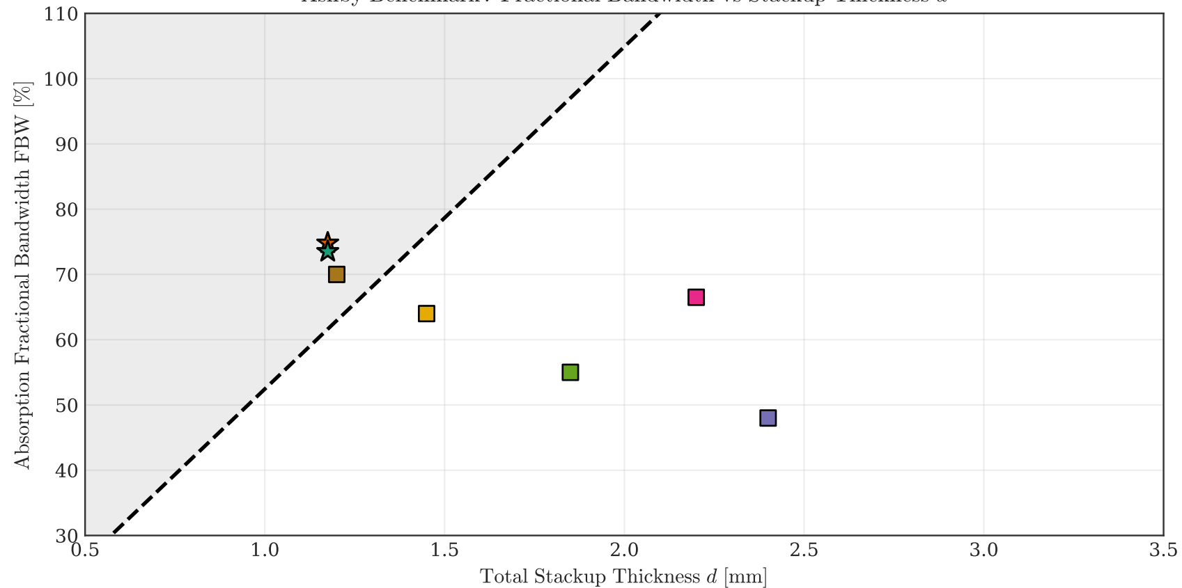
Ashby Benchmark : Fractional Bandwidth vs Stackup Thickness d
