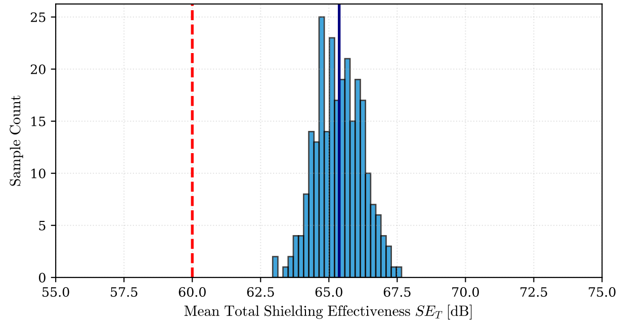
(a) Manufacturing Sensitivity : Total Shielding SE_T
