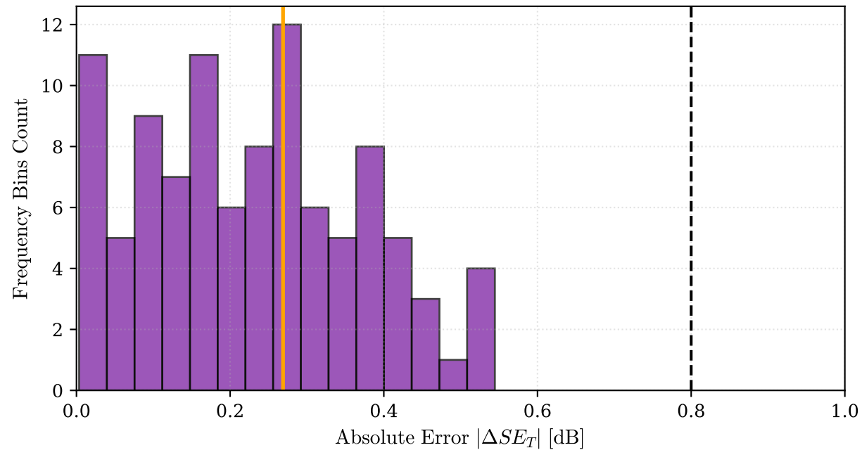
(b) Shielding Effectiveness Error Distribution
