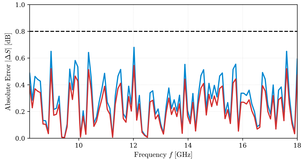
(a) Point-by-Point S-Parameter Residual Errors
