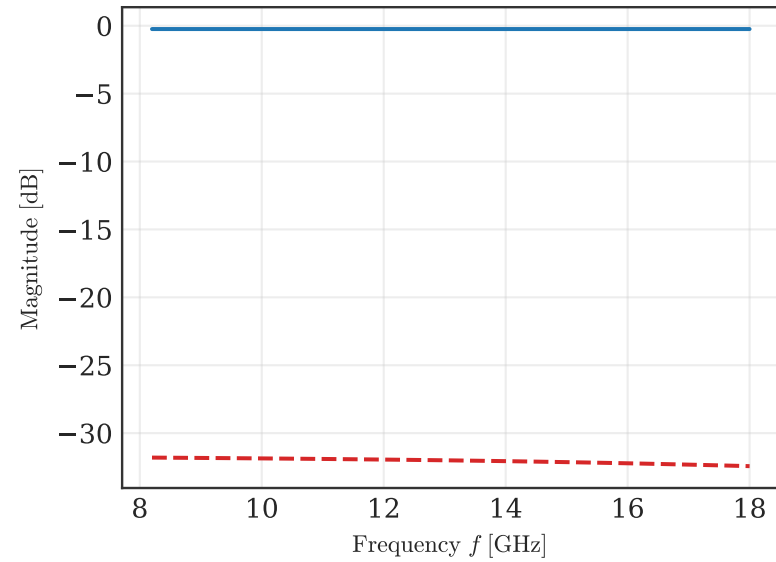
\langle SE_T \rangle = 32.0 dB
