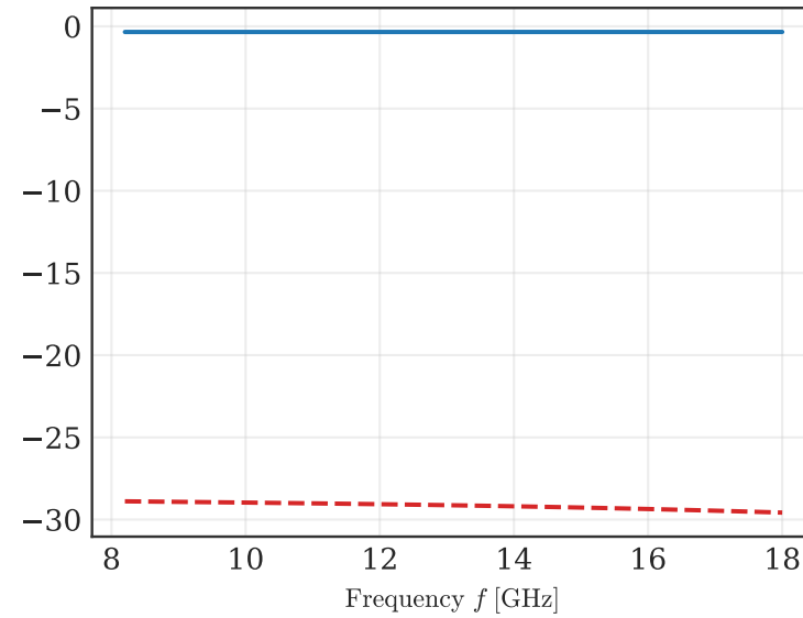
\langle SE_T \rangle = 29.2 dB
