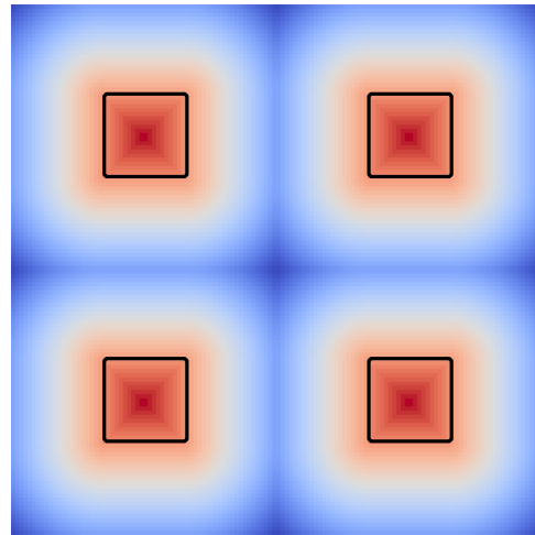
\langle SE_T \rangle = 32.0 dB
