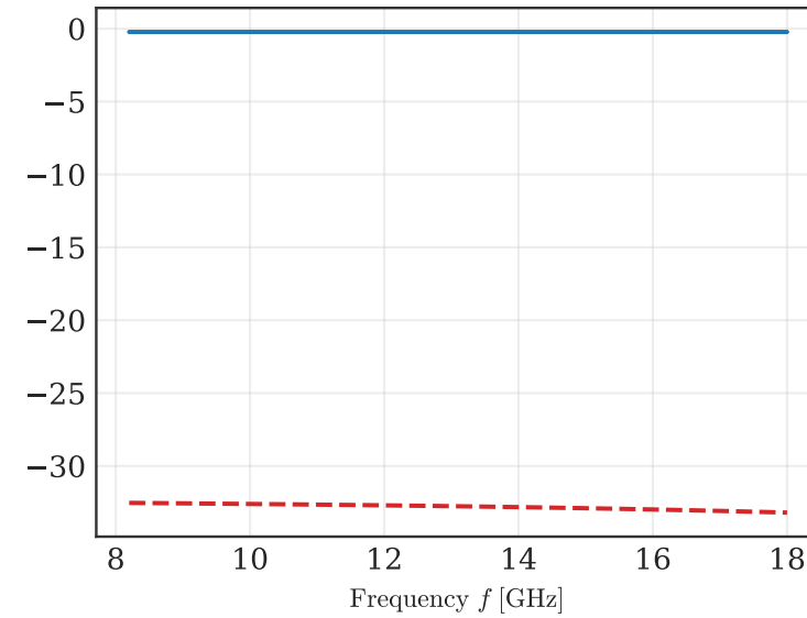
\langle SE_T \rangle = 32.8 dB
