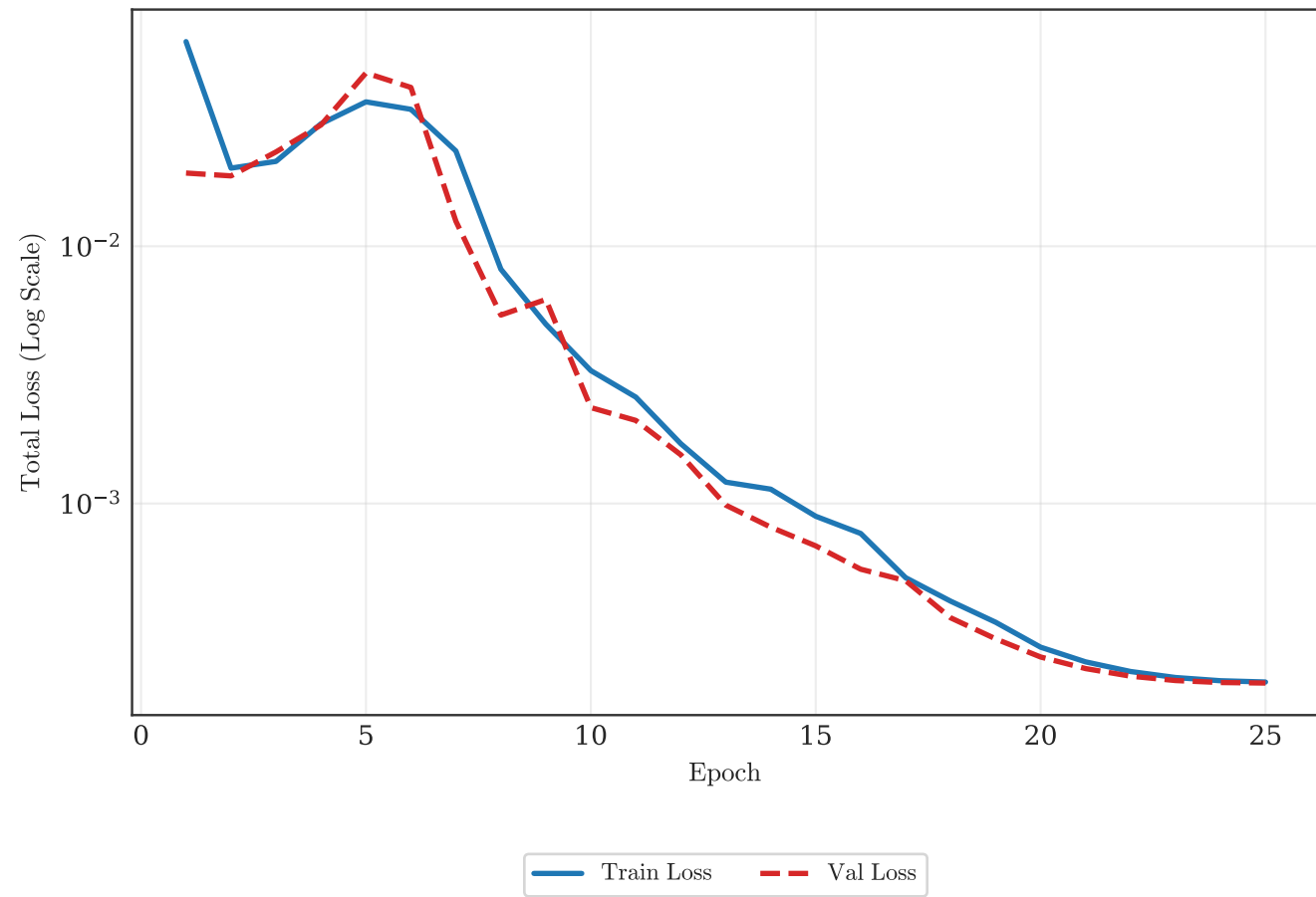
FNO Loss Convergence vs Epochs
