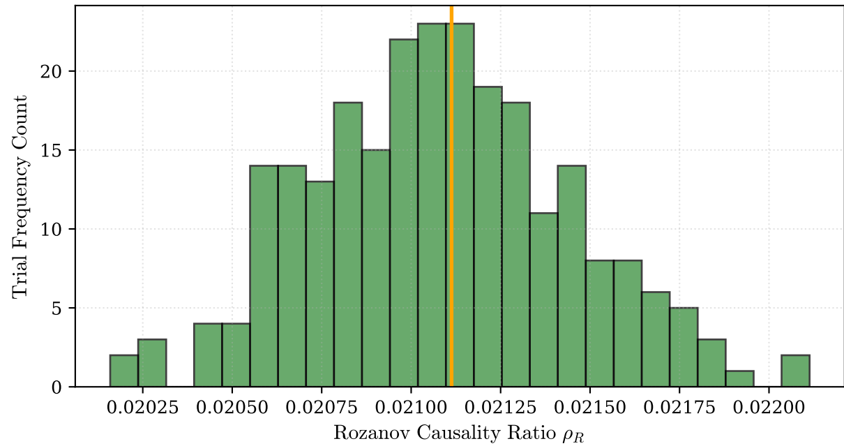
(b) Rozanov Figure of Merit Distribution \rho_R
