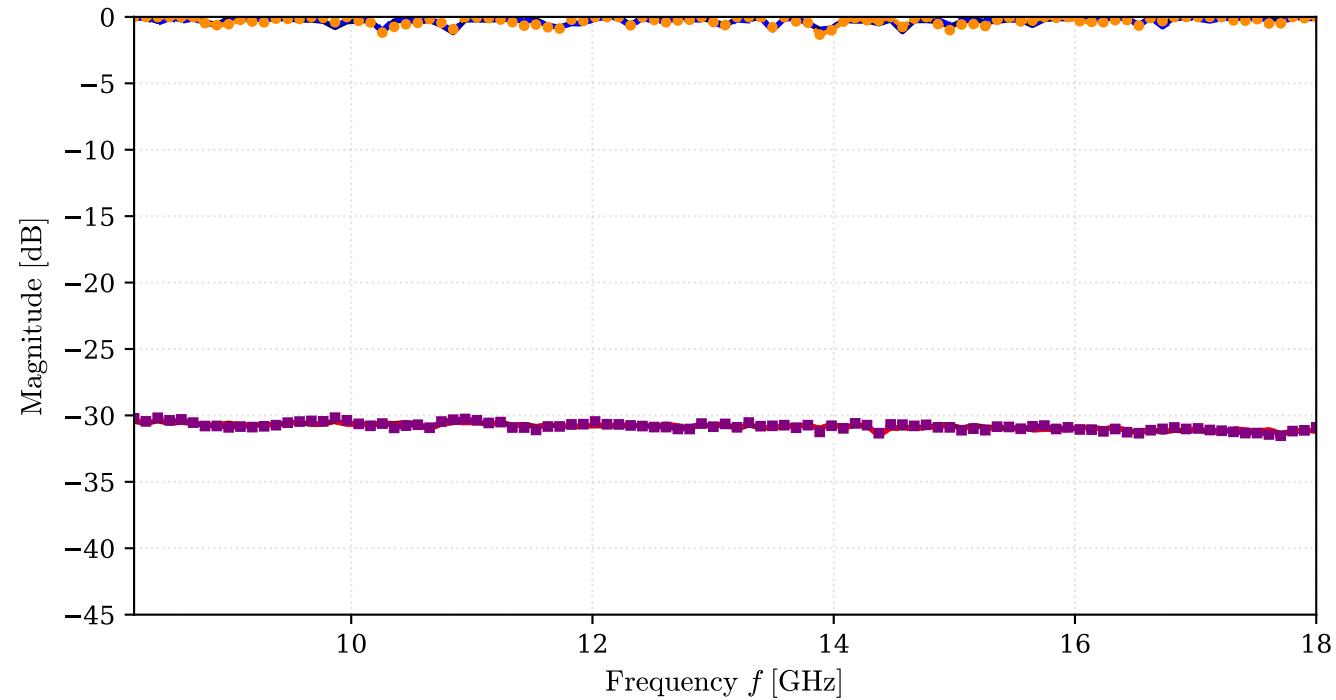
(a) Broadband Scattering Parameters ( S_{11} , S_{21} )
