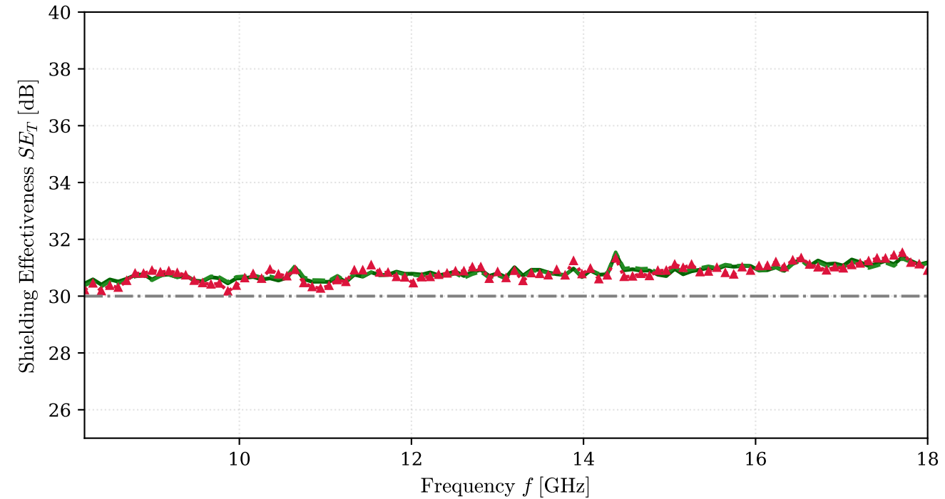
(b) Total EMI Shielding Effectiveness SE_T
