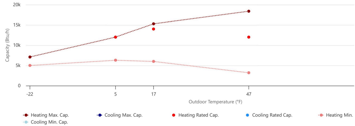
Heating/Cooling Capacity Graph
