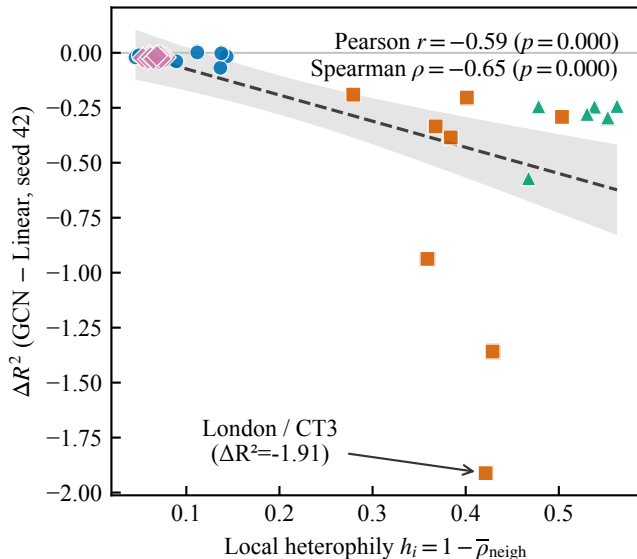
Distance topology (n=46)
