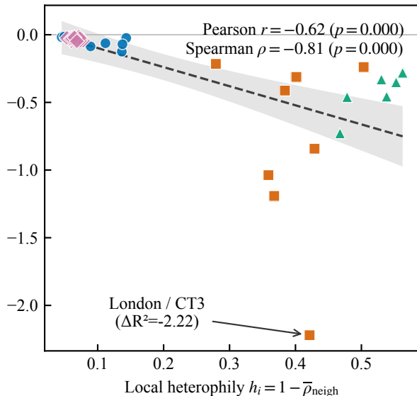
Correlation topology (n=46)
