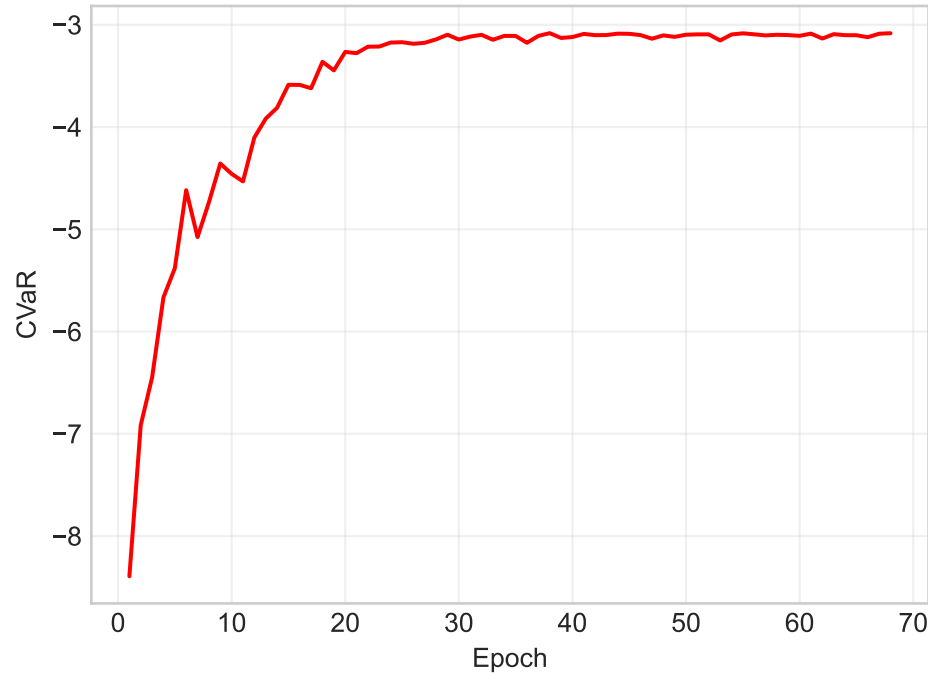
Validation CVaR
