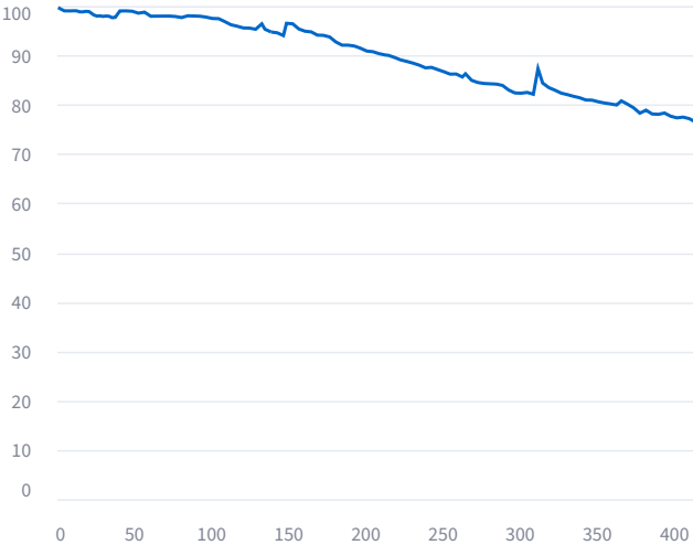
Capacity Loss (SoH Trend)
