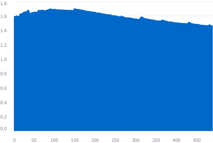
Internal Resistance Rise
