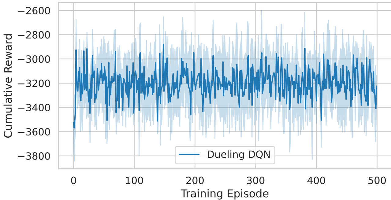
Training Convergence
