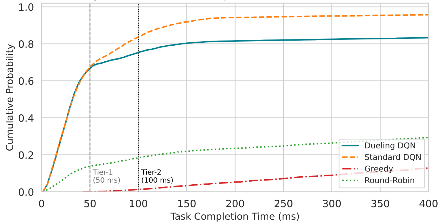
Figure 4: CDF of Task Completion Times (N = 20 devices)
