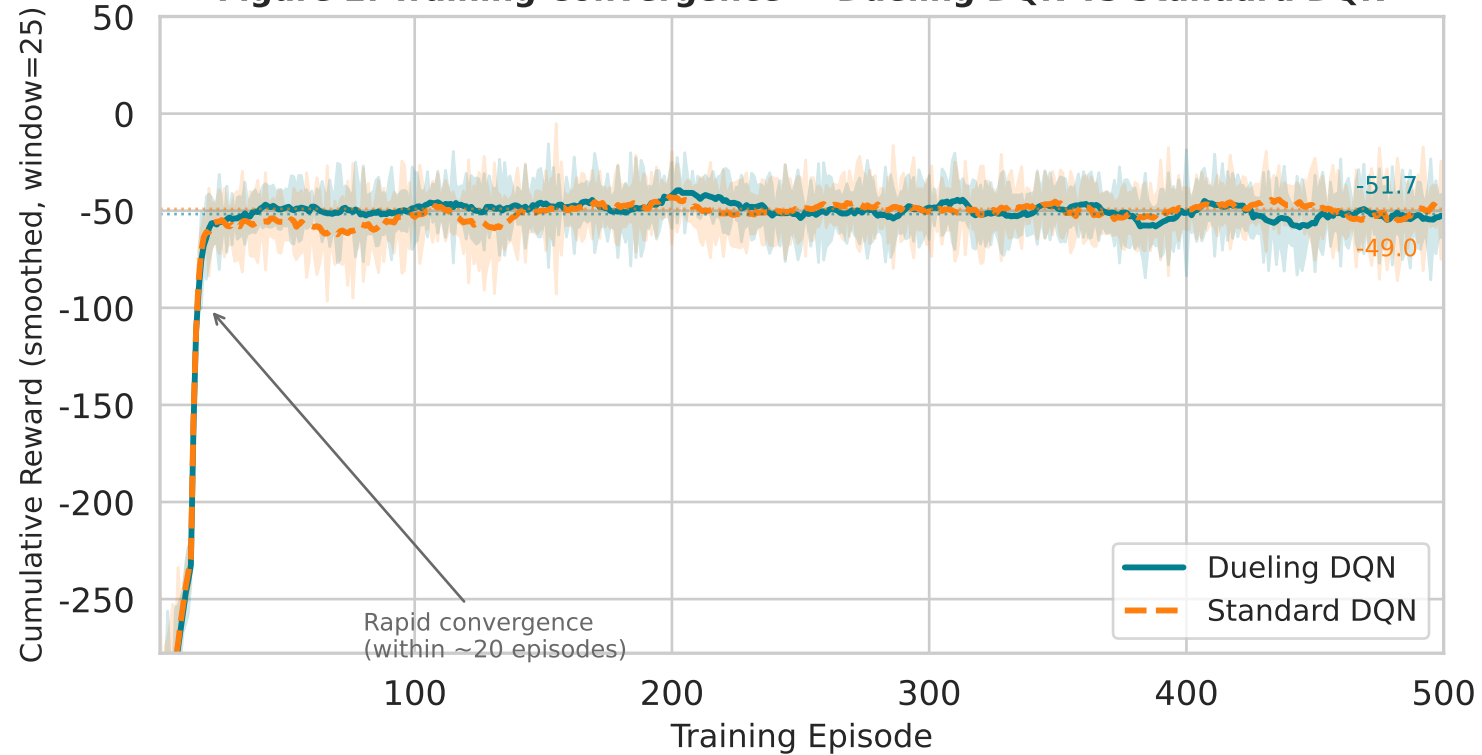
Figure 2: Training Convergence — Dueling DQN vs Standard DQN
