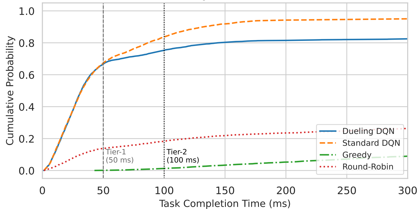
Task Completion Time CDF
