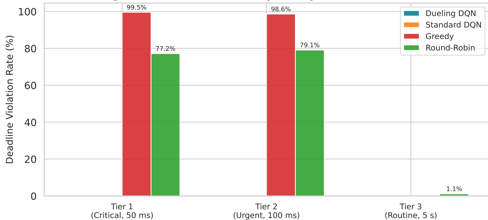
Figure 5: Deadline Violations by Priority Tier (N = 20 devices)
