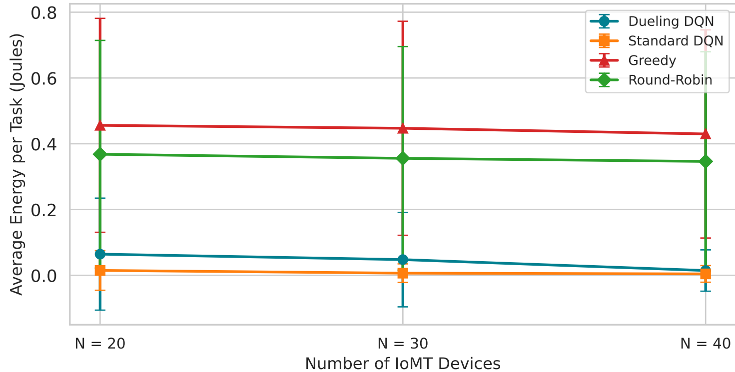
Figure 6: Scalability — Energy Consumption vs Device Count
