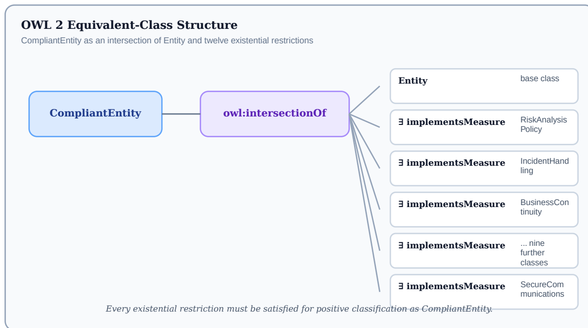
Figure 6.2: OWL equivalent-class structure for CompliantEntity
