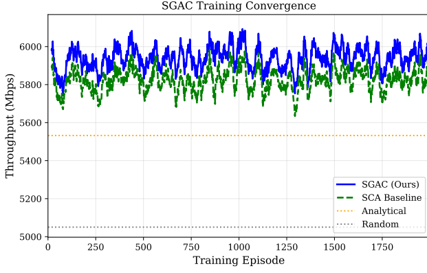
Fig. 2: Training convergence over 2000 episodes. SGAC (blue) consistently exceeds SCA baseline (green dashed) and significantly outperforms random (gray) and analytical (orange) heuristics.
