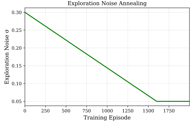
Fig. 7: Exploration noise \sigma annealing during training. The schedule transitions from exploratory behavior ( \sigma = 0.3 ) to exploitation ( \sigma = 0.05 ) over the training horizon.
