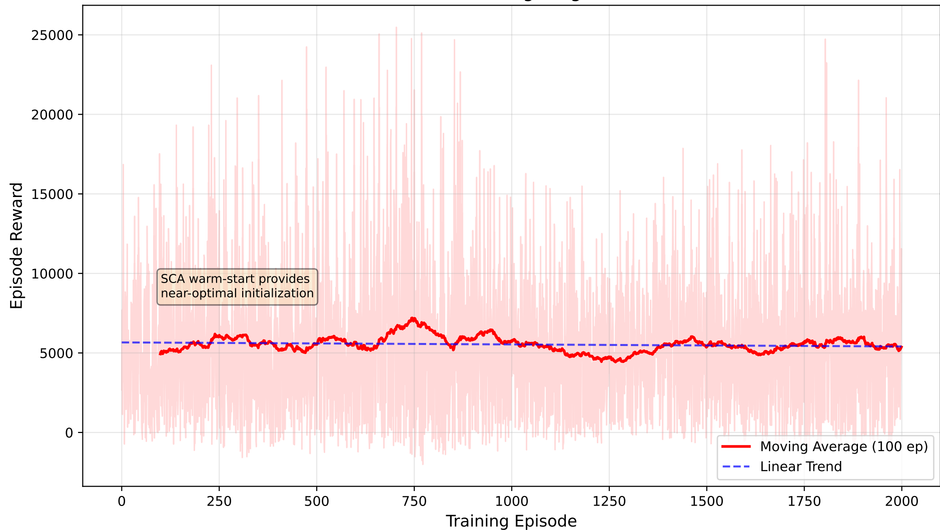
SGAC Training Progress
