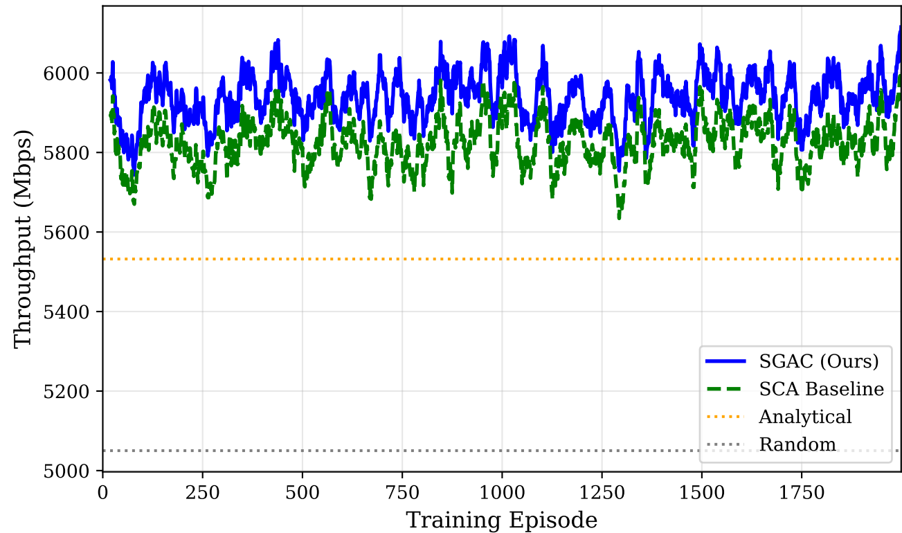
SGAC Training Convergence
