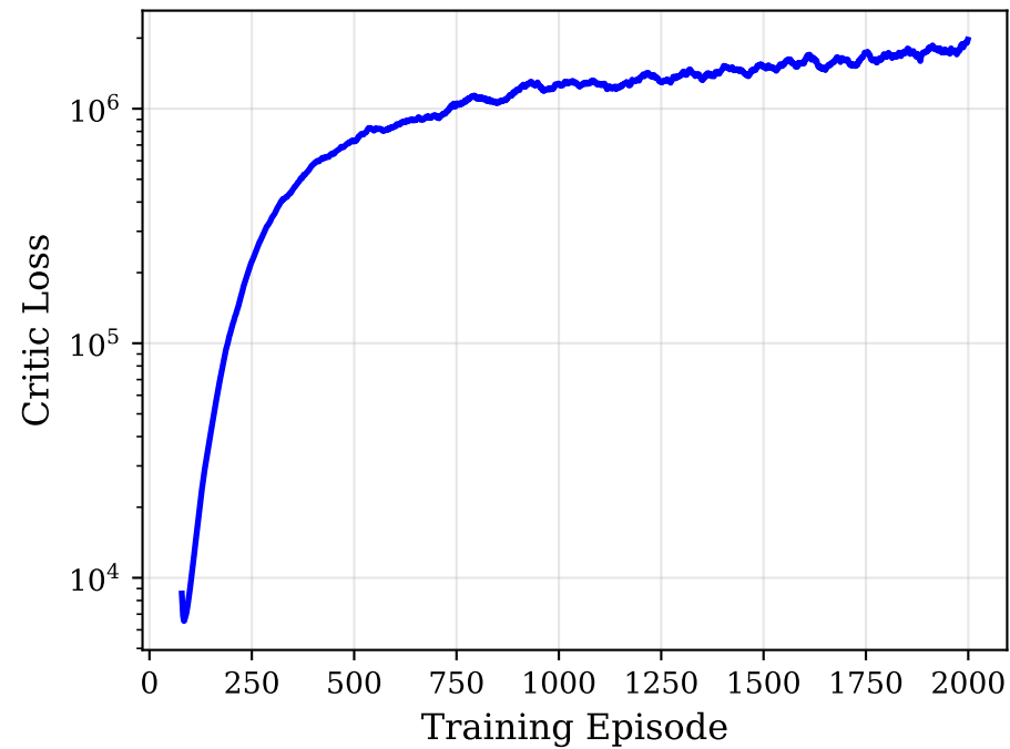
Twin Critic Loss
